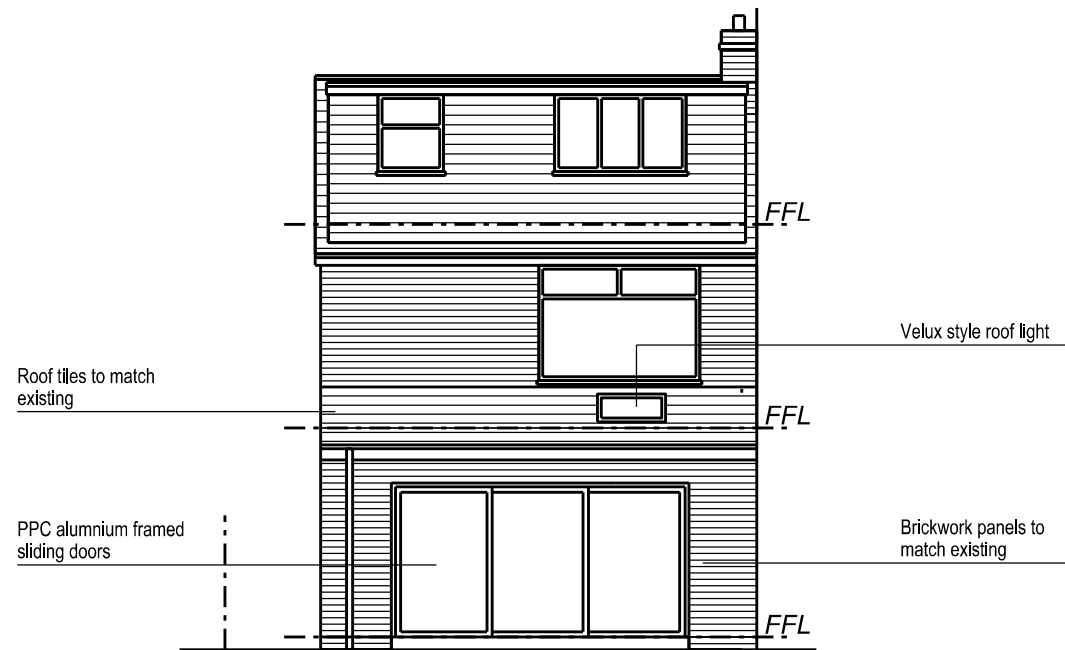
West Elevation
