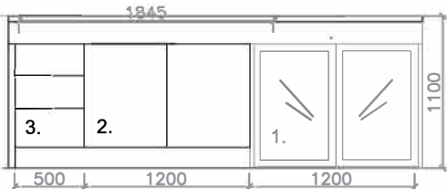
South Elevation scale 1/50
