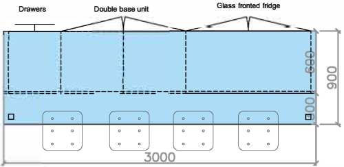
Plan View Scale 1/50
