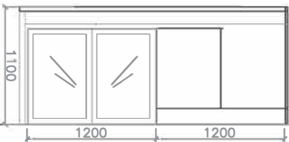
North Elevation scale 1/50
