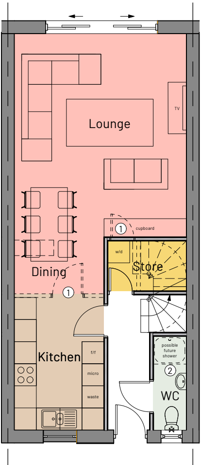
1 Ground Floor Plan (Typical Townhouse) Scale: 1:100
