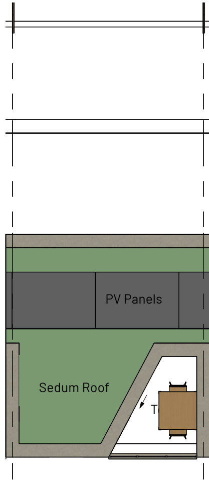
4 Roof Plan (Typical Townhouse) Scale: 1:100
