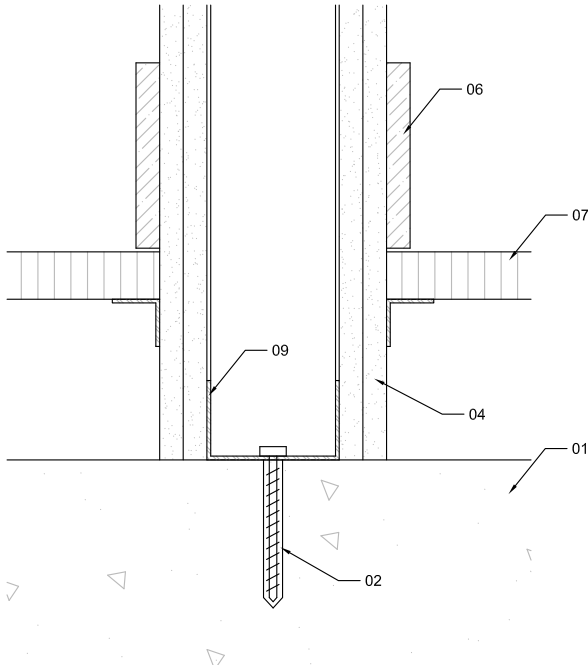
Lobby Wall - Base Detail
