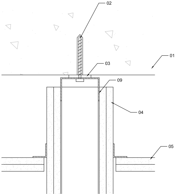
Lobby Wall - Head Detail
