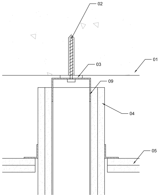
Demising Wall - Head Detail
