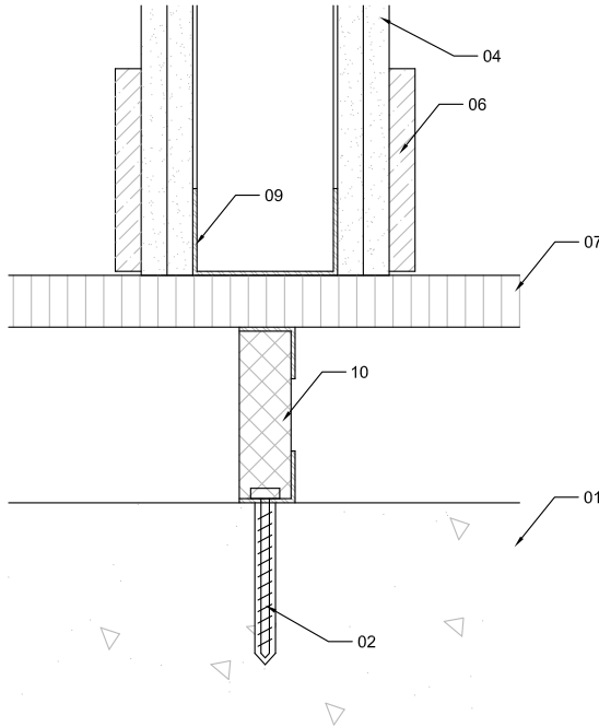
Demising Wall - Base Detail
