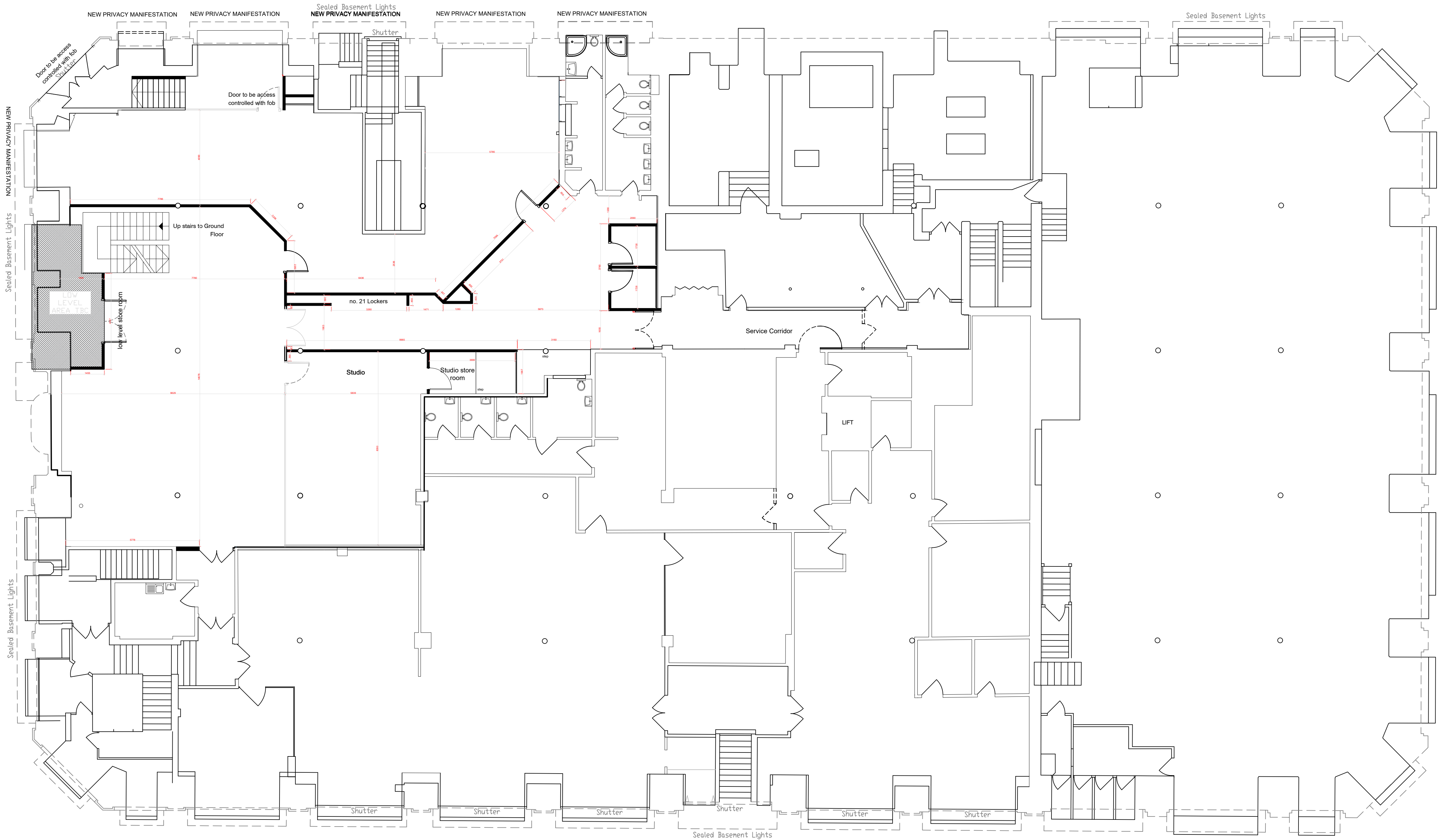
Lower Ground Floor - Setting Out Drawing Scale 1:100
