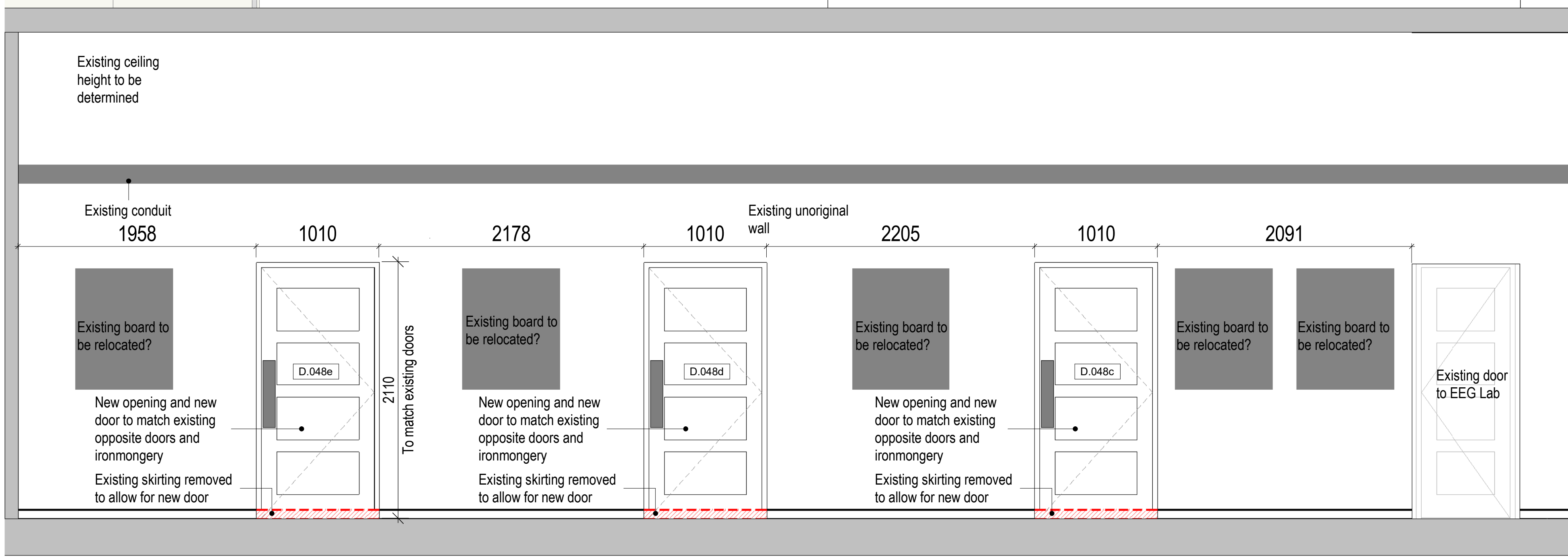
G.048C EEG Lab Corridor Elevation as Proposed
