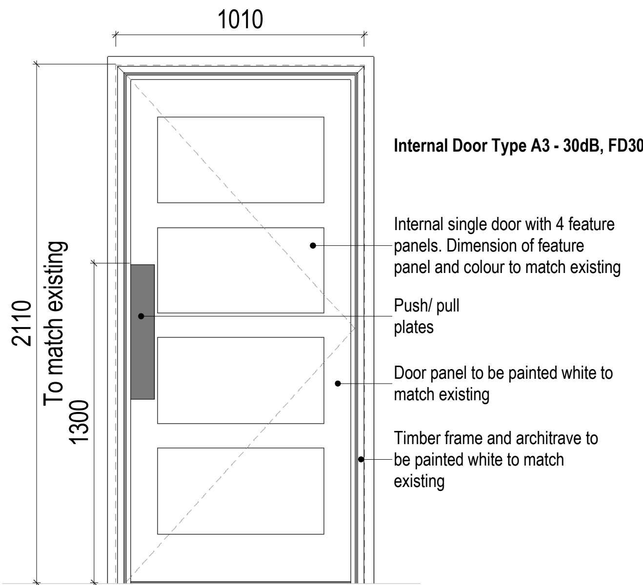
Proposed Door Elevation
