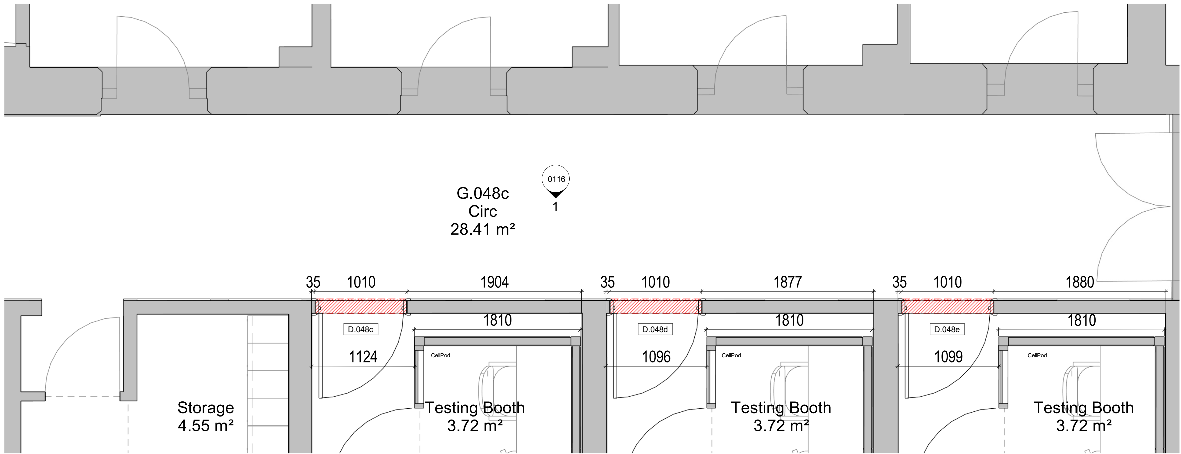
L0 Zochonis Occupation - G.048c EEG Lab Corridor as Proposed
