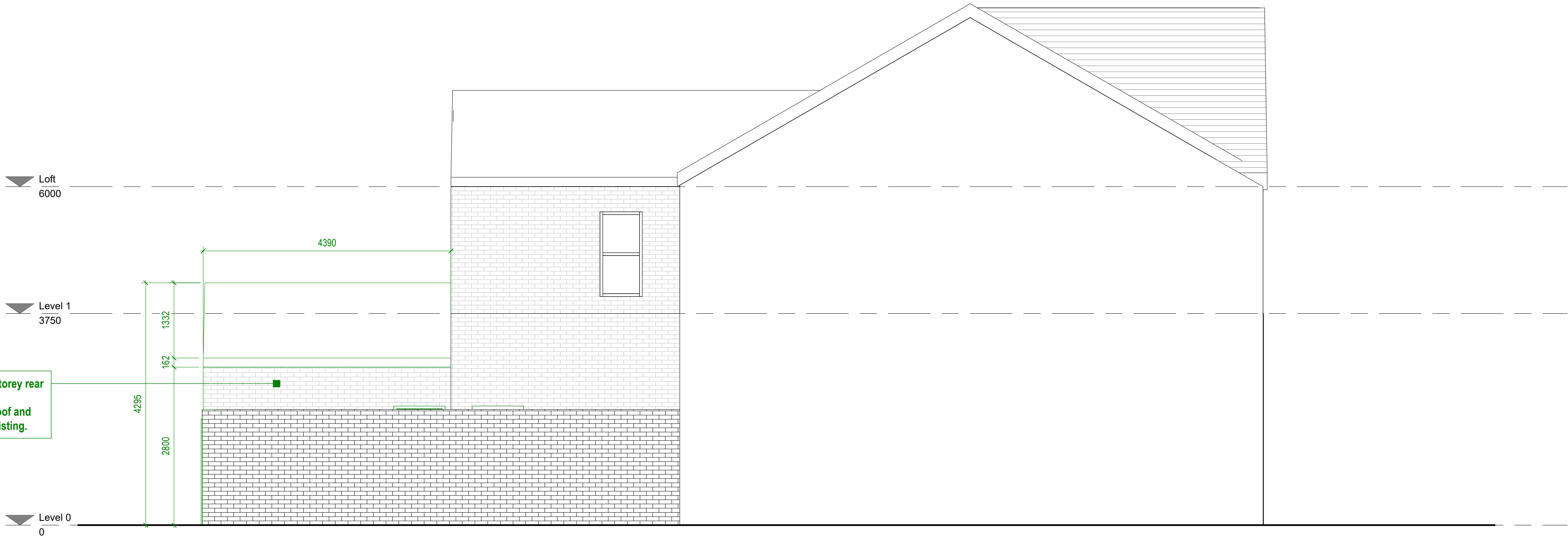
2 Proposed Side 1 Elevation 1 : 50
