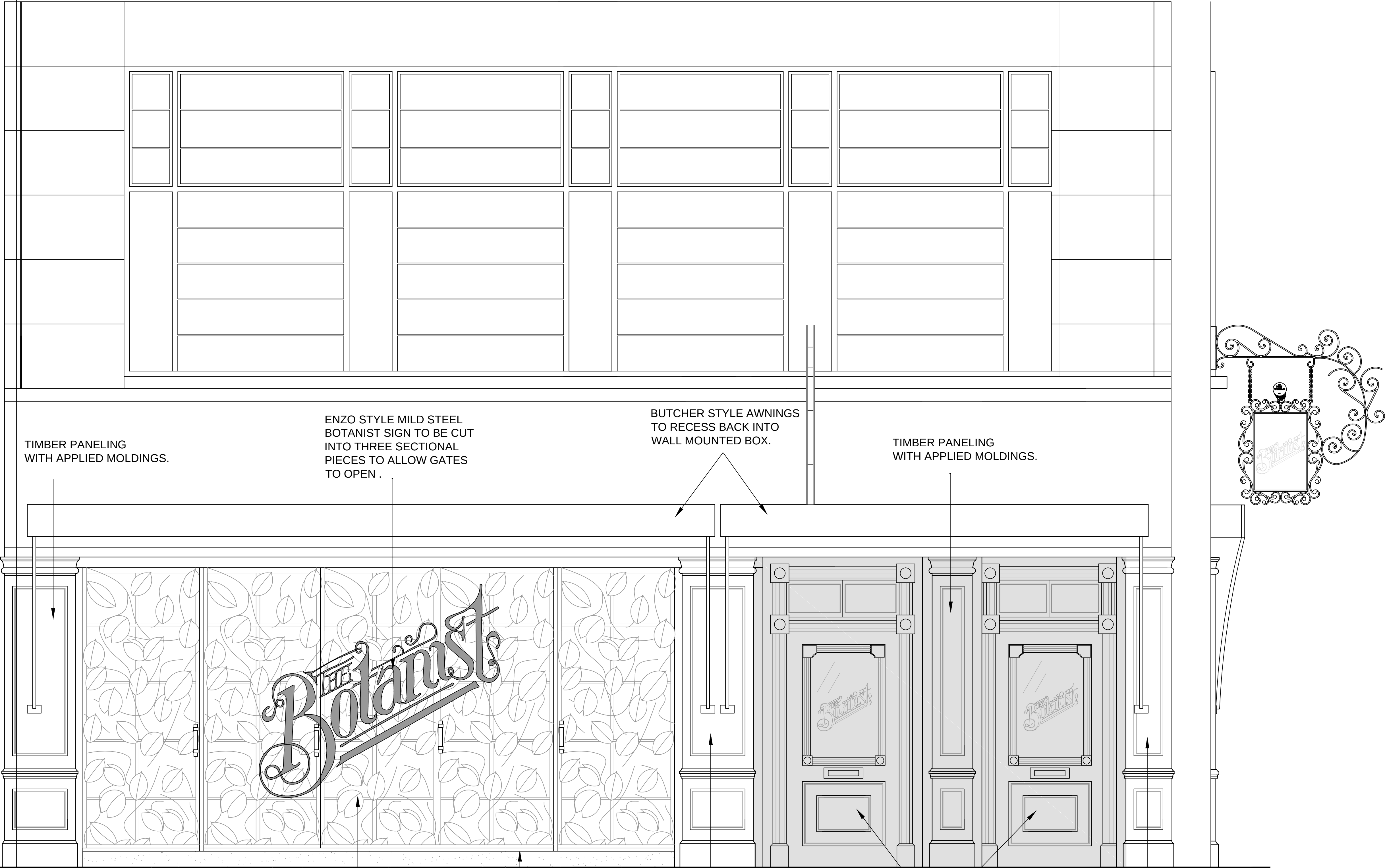
DEANSGATE ELEVATION.
