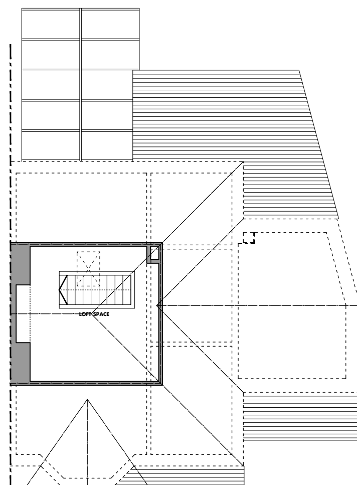
EXISTING LOFT PLAN
