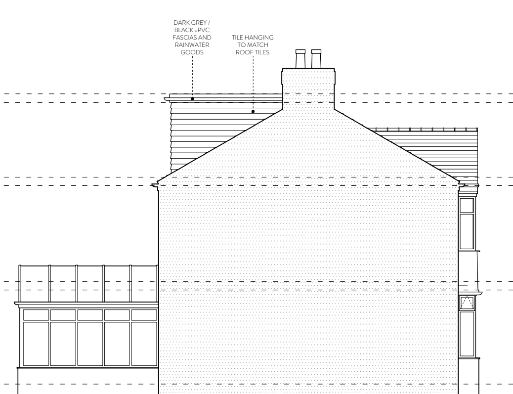
PROPOSED SIDE ELEVATION (PARTY WALL)
