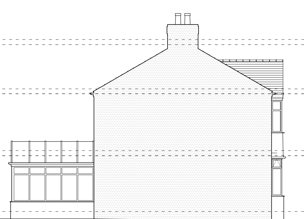
EXISTING SIDE ELEVATION (PARTY WALL)
