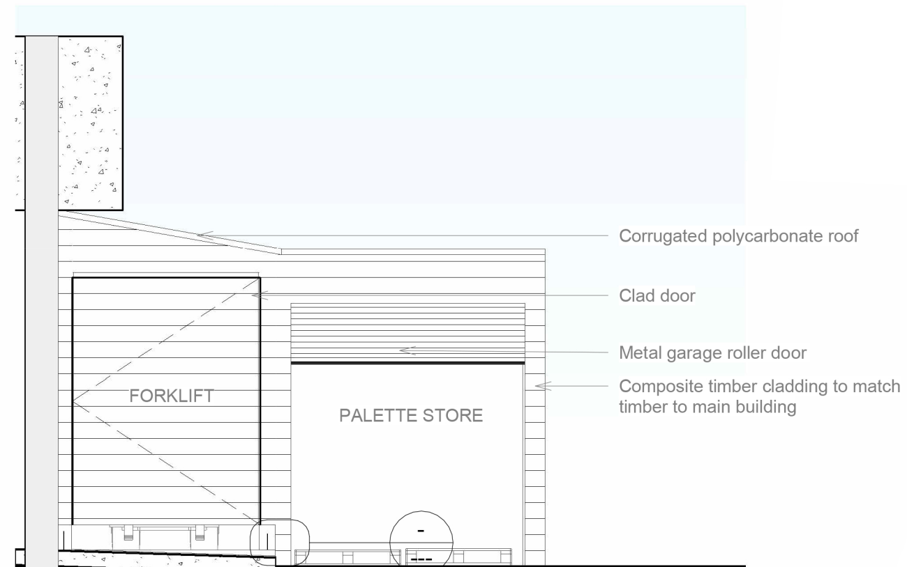
West Elevation to Manchester Road 1 : 50
