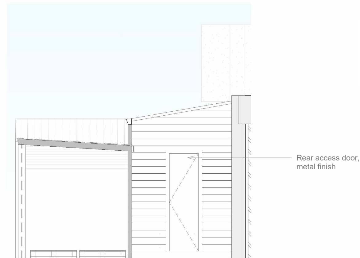
South Elevation 1 : 50
