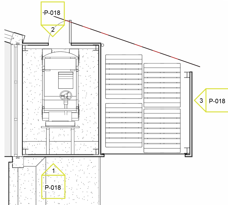
Proposed Plan 1 : 50
