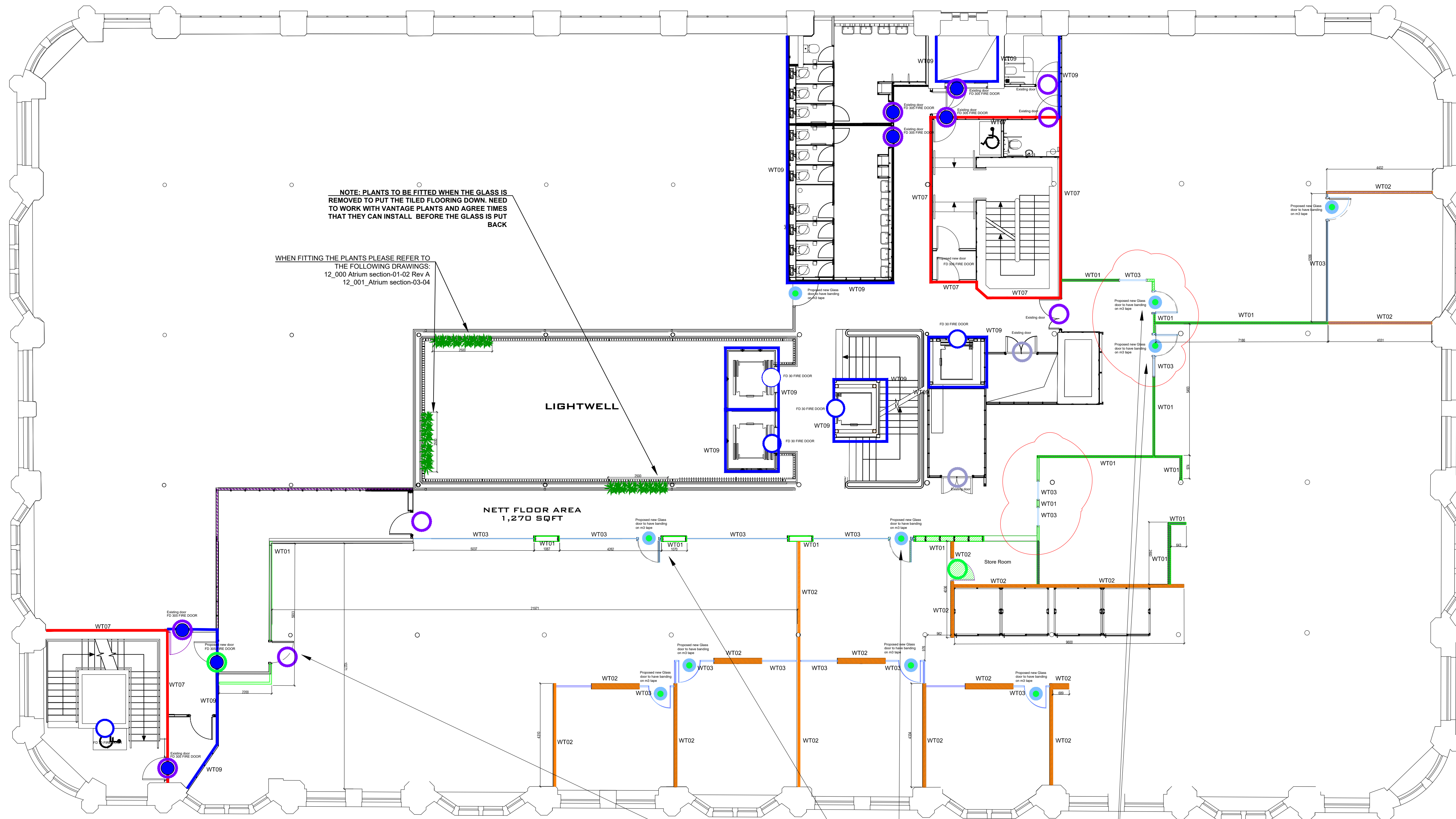
First Floor - Wall Types Scale 1:100
