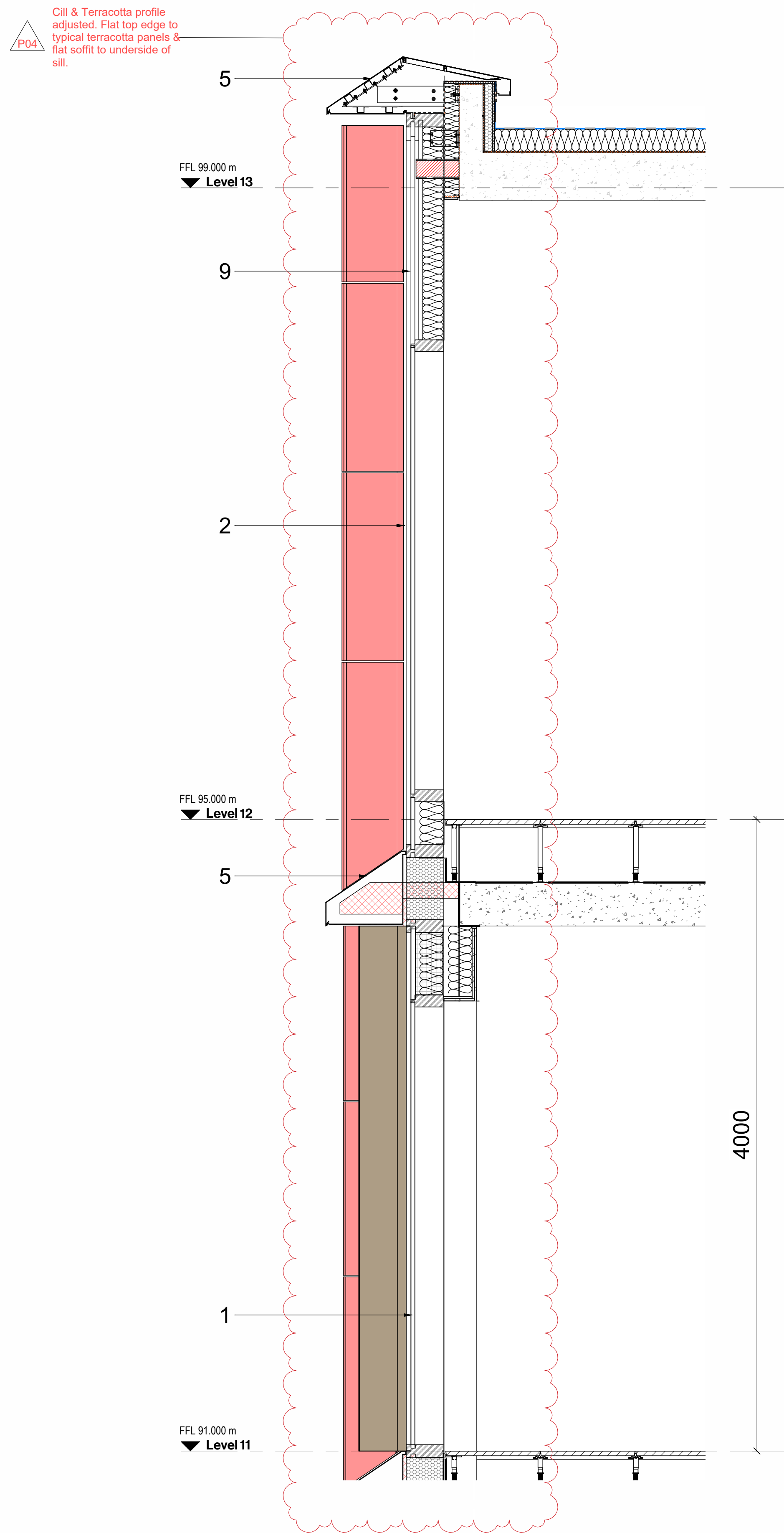
2 Roof Bay Study Section
