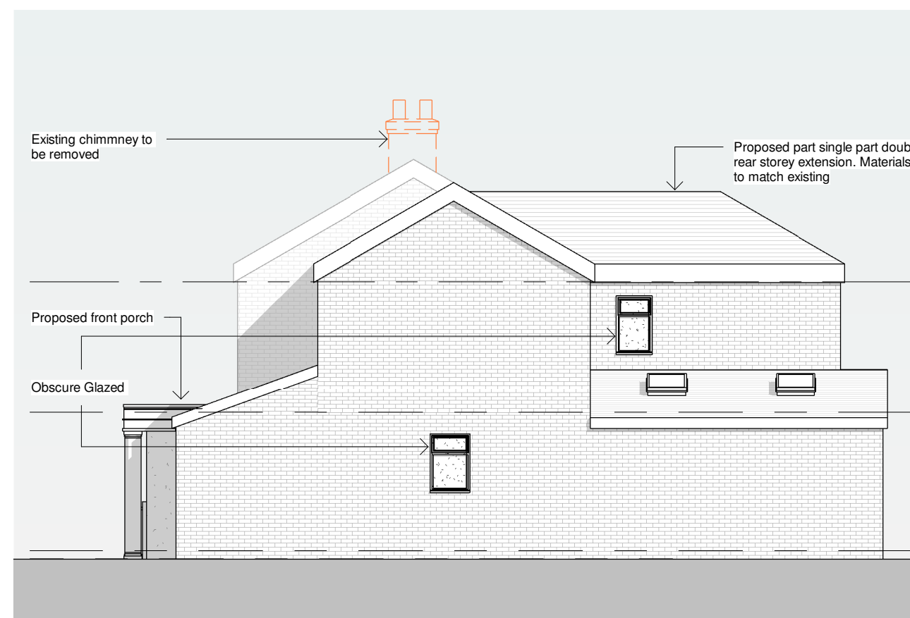
4 Proposed West Elevation 1 : 100
