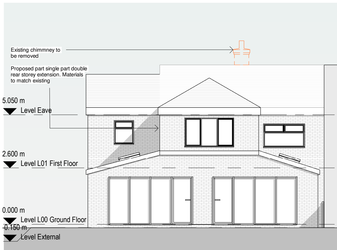
3 Proposed South Elevation 1 : 100
