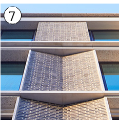
Reconstituted stone banding/coping detail
