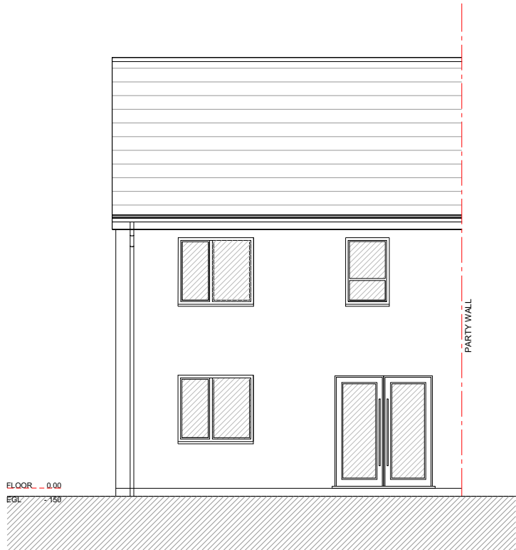
REAR ELEVATION
