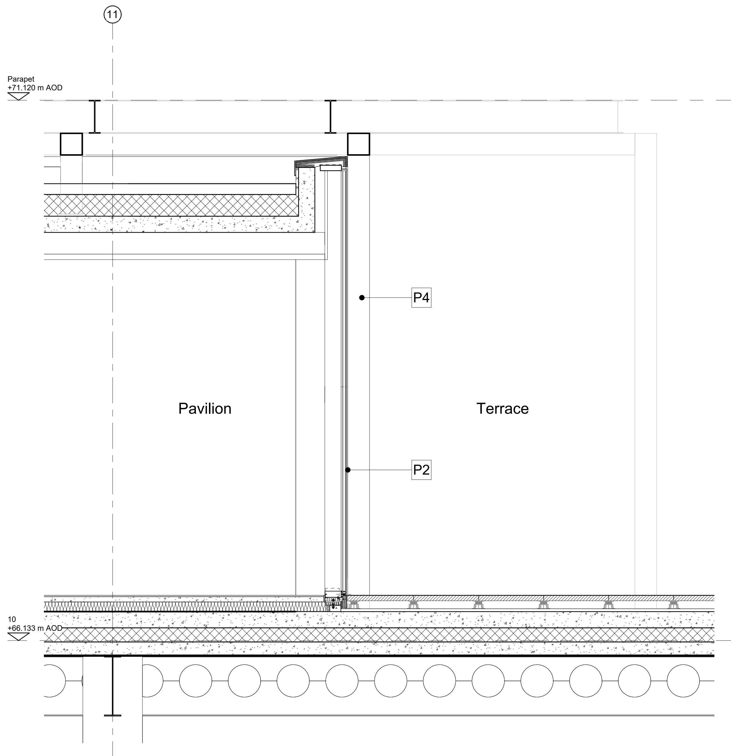
Scale 1:20 @ A1
