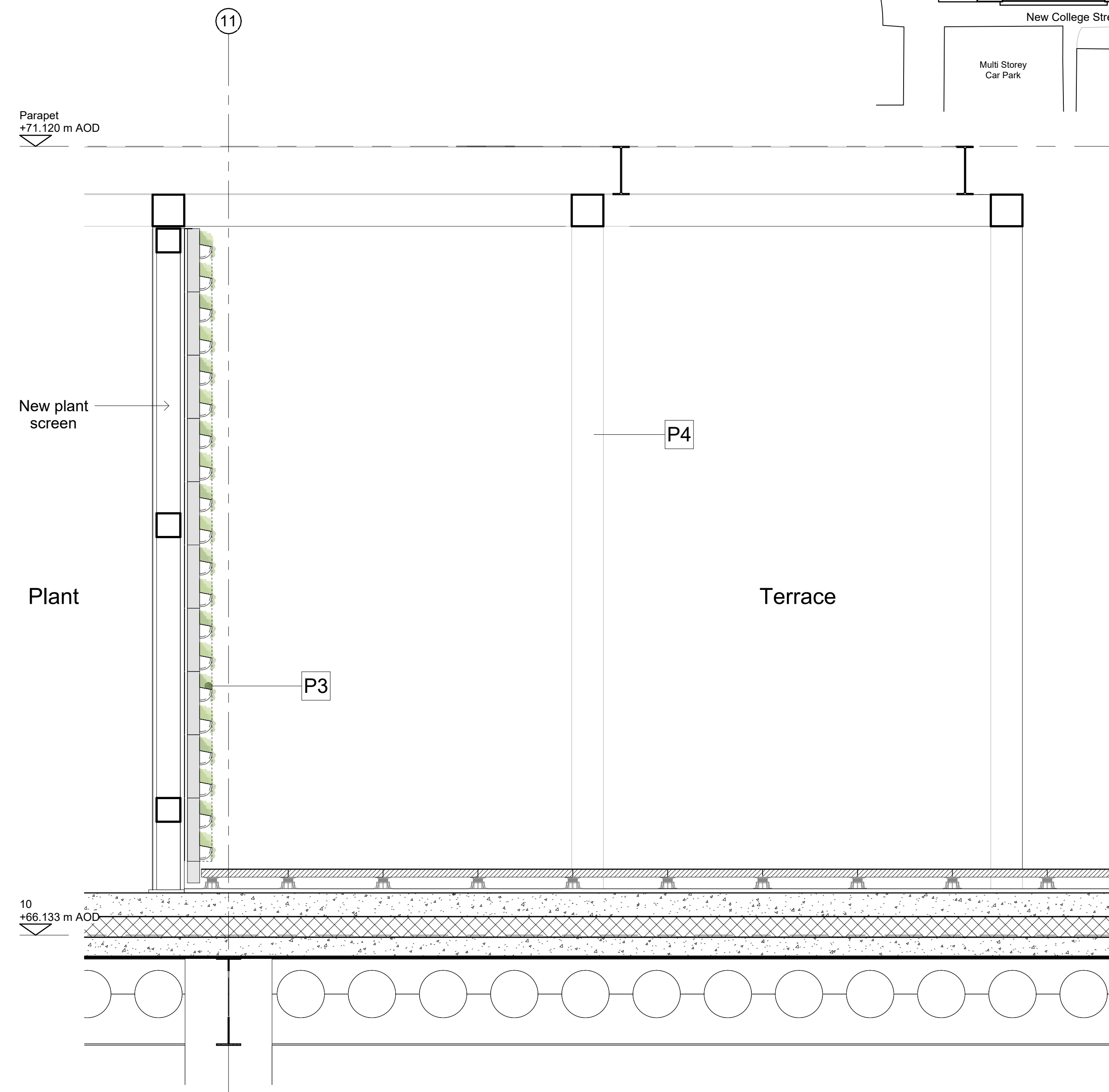
Scale 1:20 @ A1
