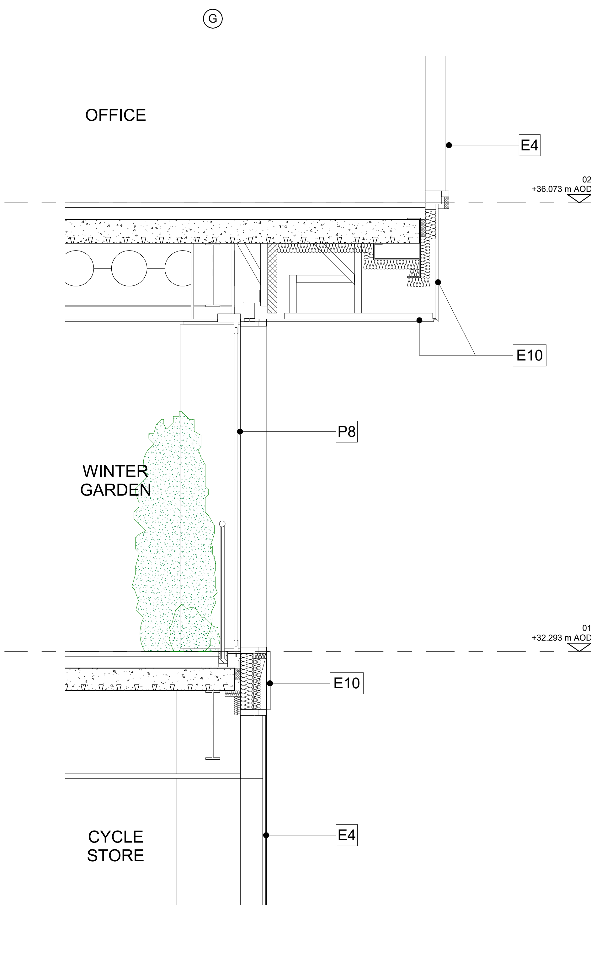
Detailed Section EE - Proposed L01 South Facade Scale 1:20 @ A1
