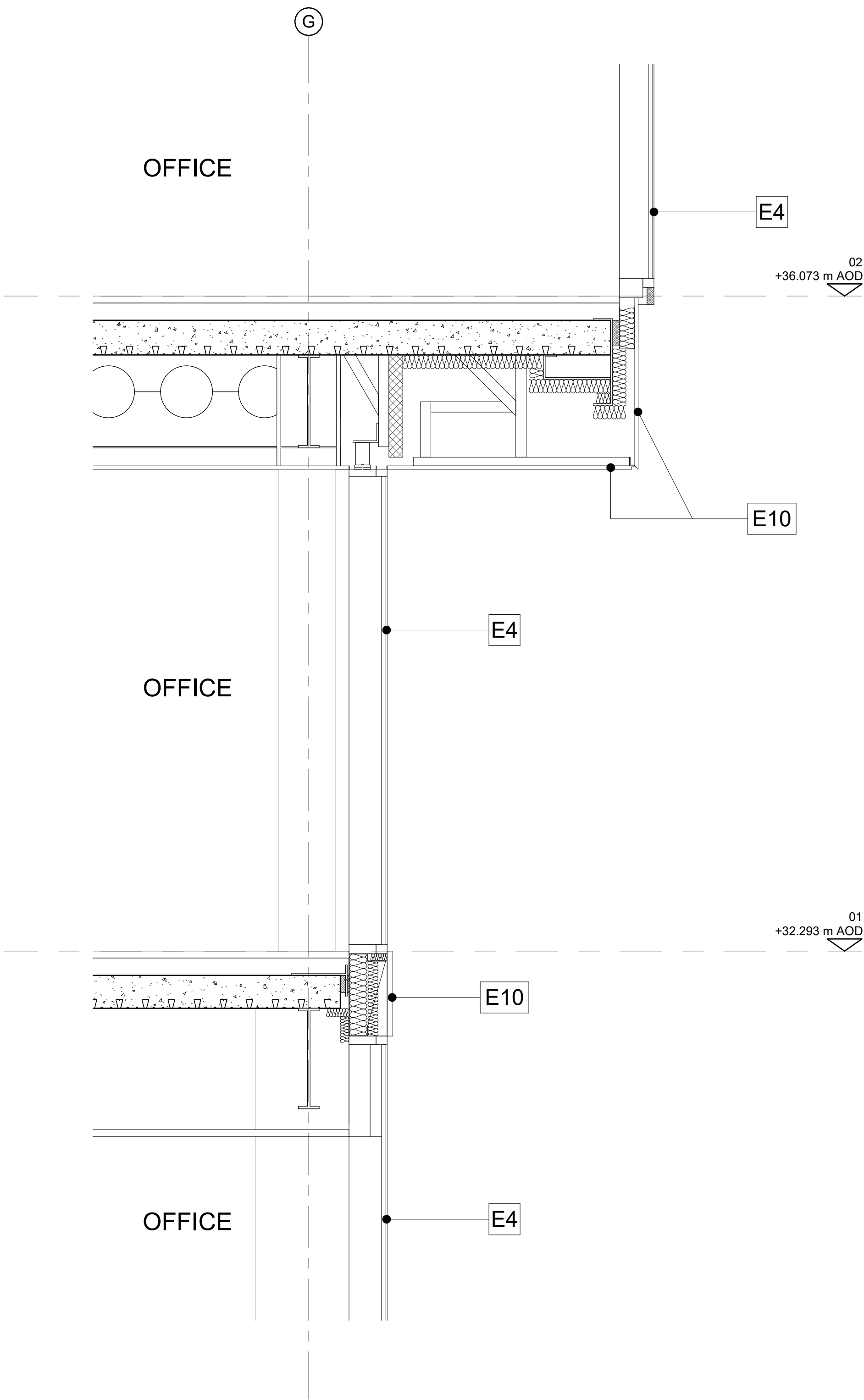
Detailed Section EE - Existing L01 South Facade Scale 1:20 @ A1
