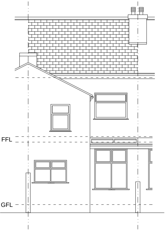
Existing/ Proposed Rear Elevation
