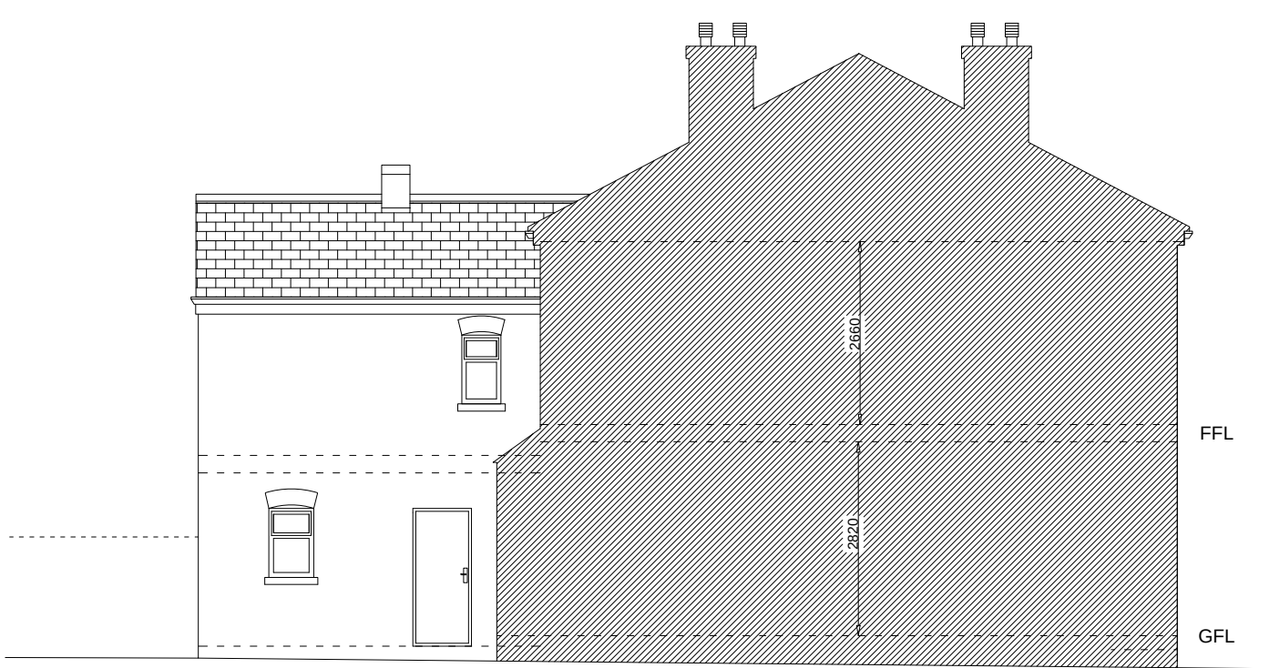
Existing/ Proposed LHS Elevation
