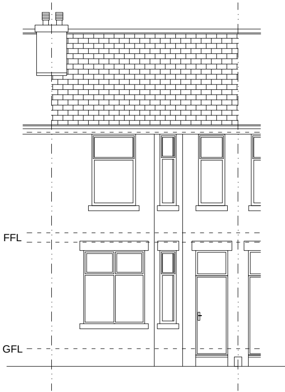
Existing/ Proposed Front Elevation
