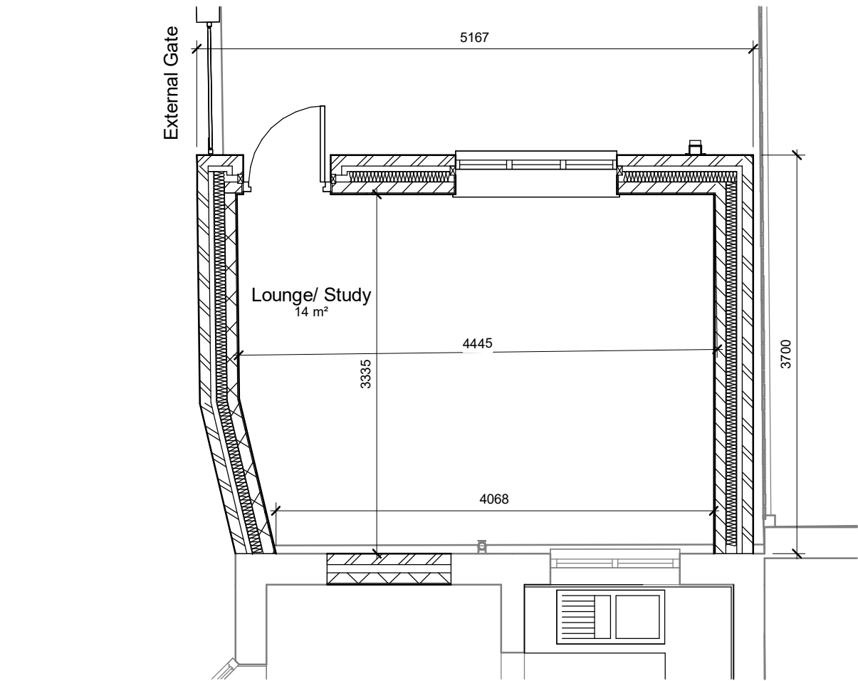
Proposed- Ground Floor - Opt. 2 1 : 50
