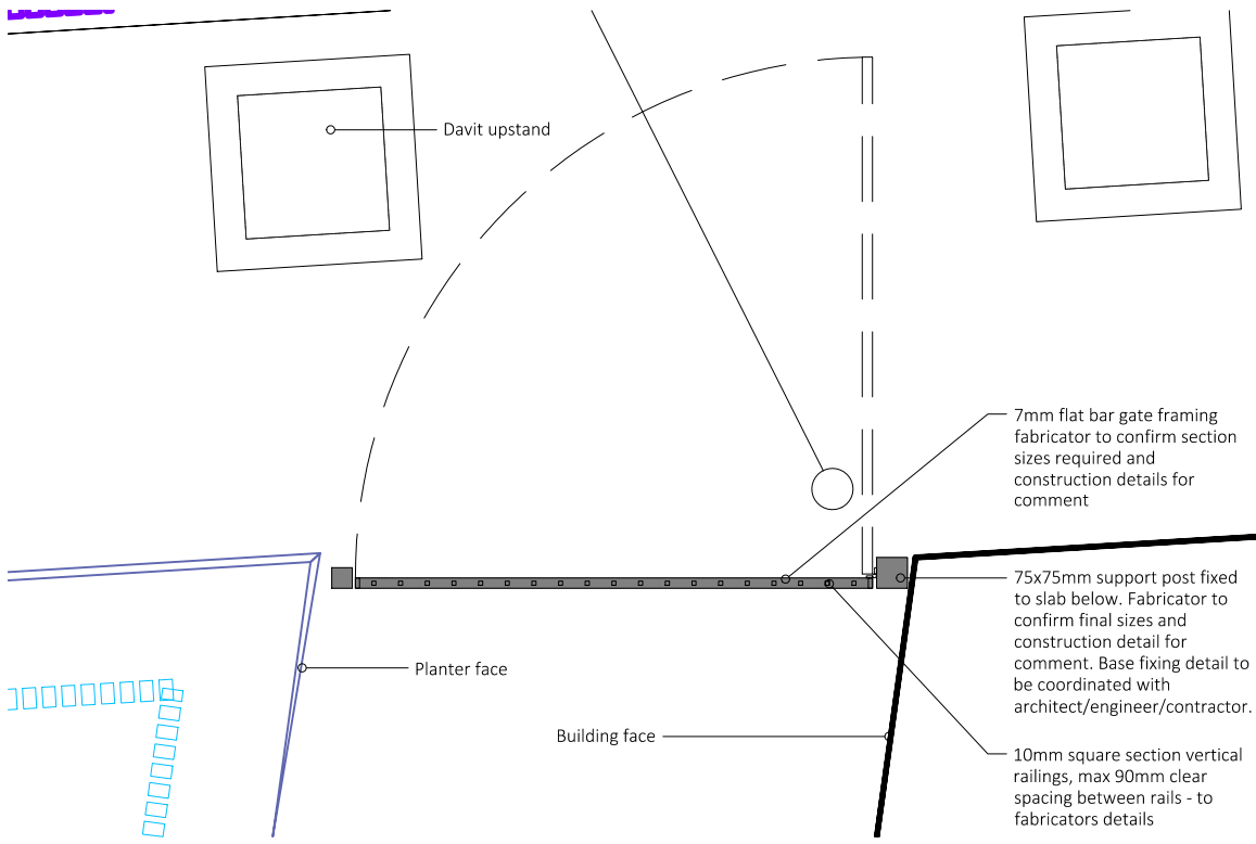
PLAN VIEW 2 - Type 2 Gate 1:20
