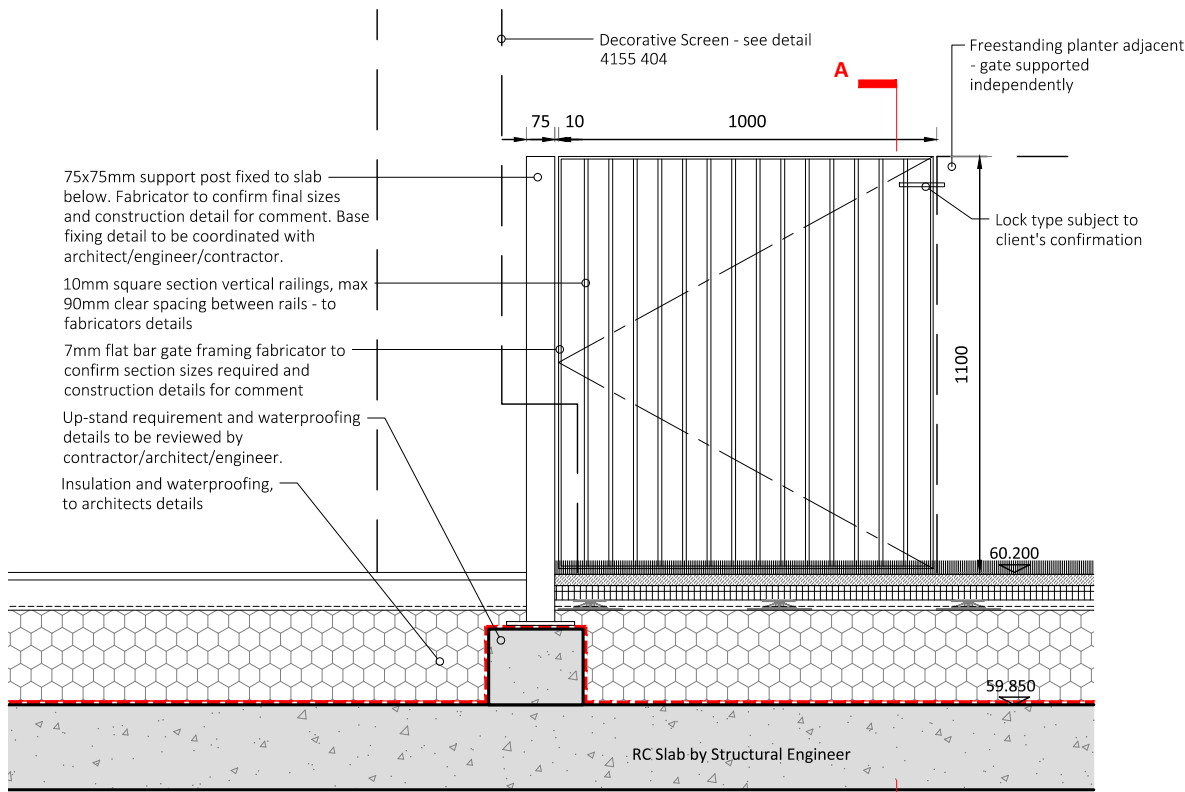
ELEVATION 1 - Type 1 Gate 1:20
