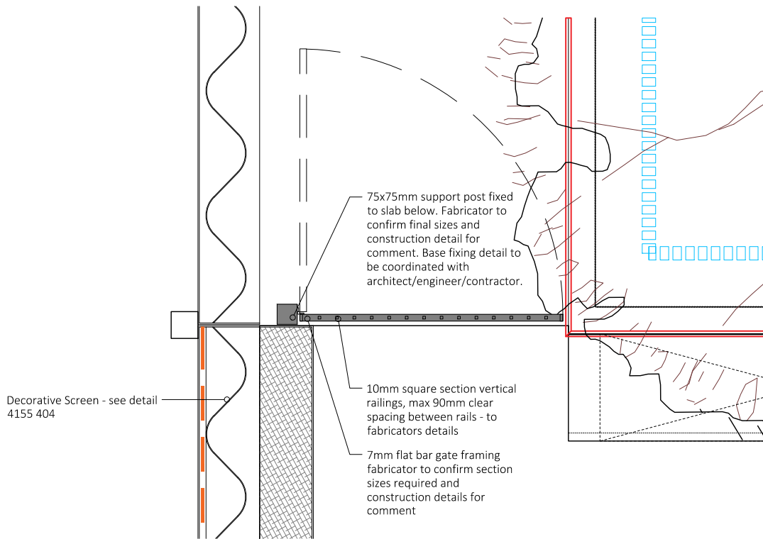
PLAN VIEW 1 - Type 1 Gate 1:20
