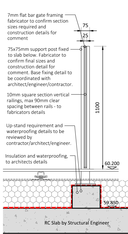
SECTION A-A - Type 1 & 2 Gate 1:20
