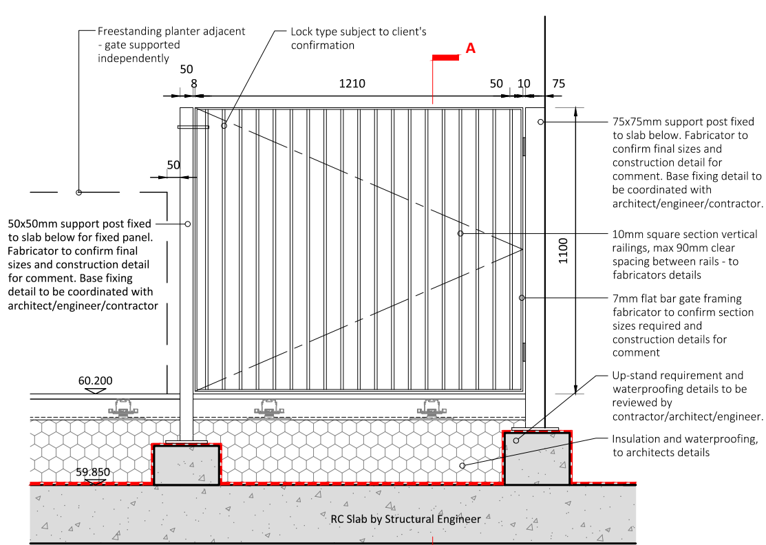
ELEVATION 2 - Type 2 Gate 1:20
