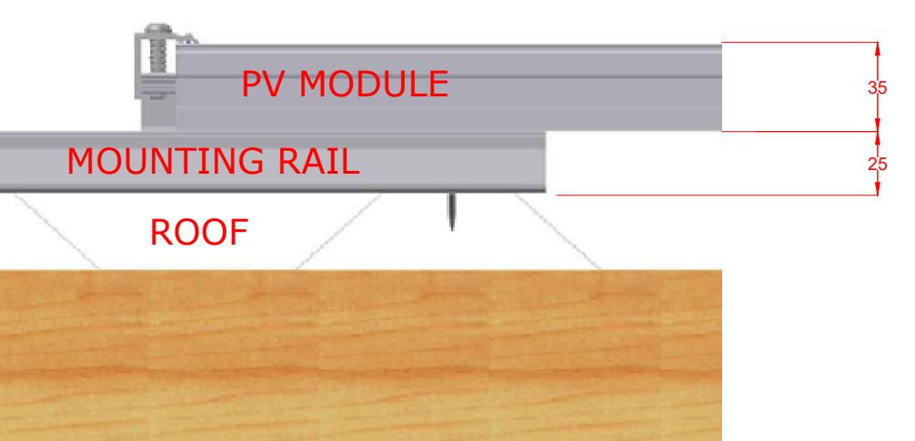
PV MODULE FIXING
