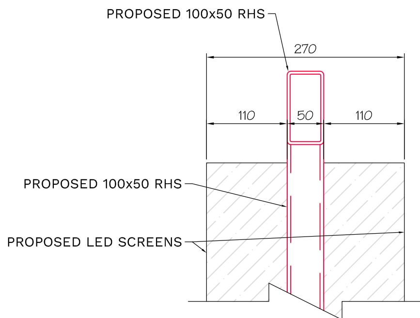
PROPOSED TYPICAL PART SECTION THROUGH NEW LED SCREEN (SCALE 1:5 AT A1)
