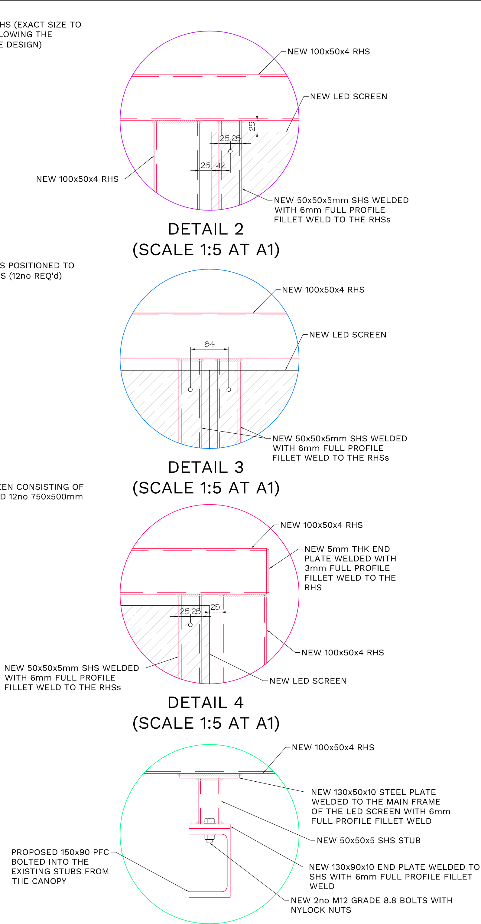
DETAIL 5 (SCALE 1:5 AT A1)
