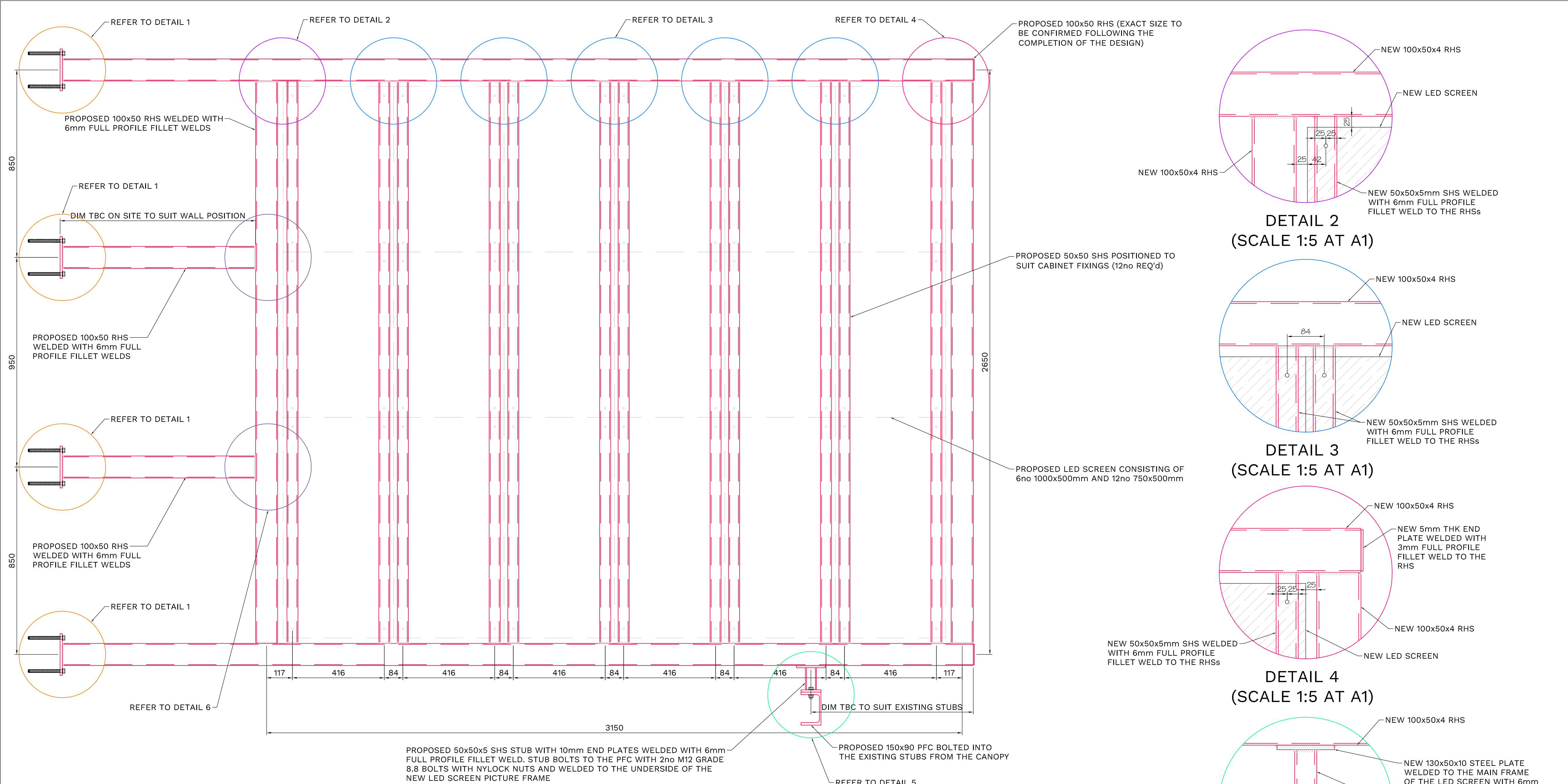
PROPOSED ELEVATION ON NEW SUPPORTING STEELWORK (SCALE 1:10 AT A1)
