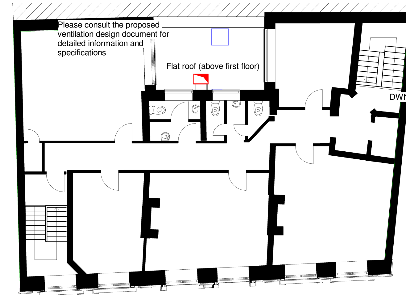
Proposed Third Floor 1 : 100
