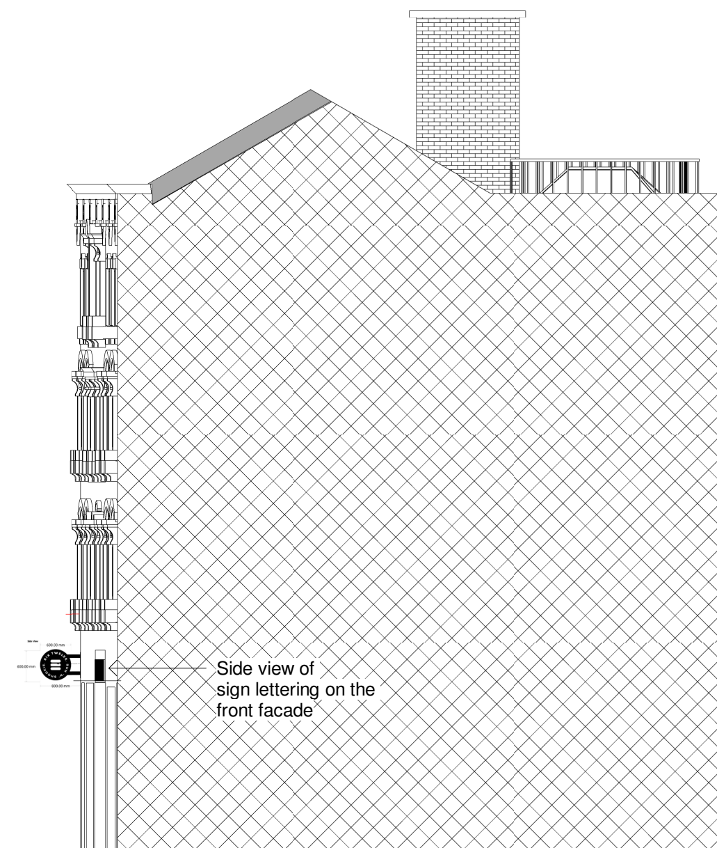
Proposed Side 1 : 100
