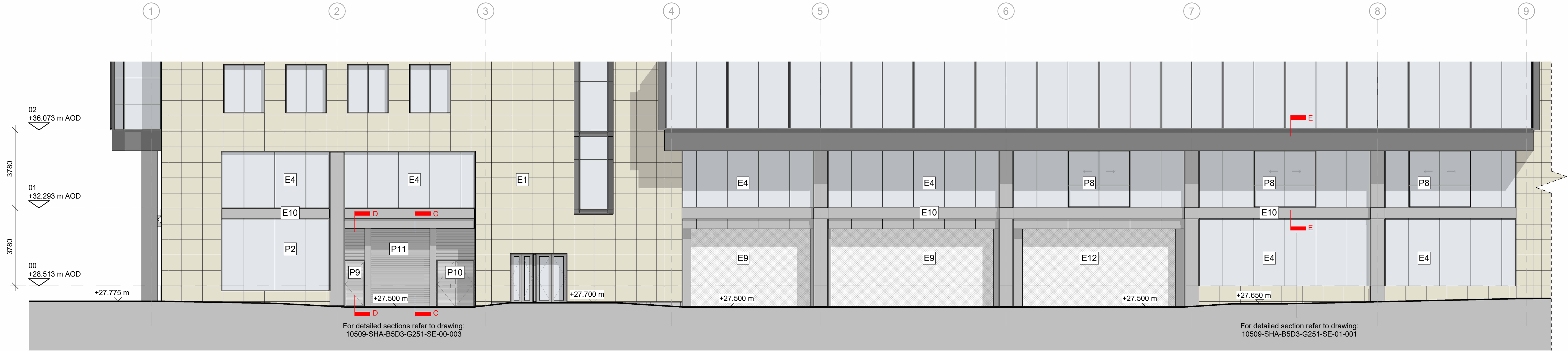
Proposed Ground Floor - South Elevation (1 of 2) (New College St)
