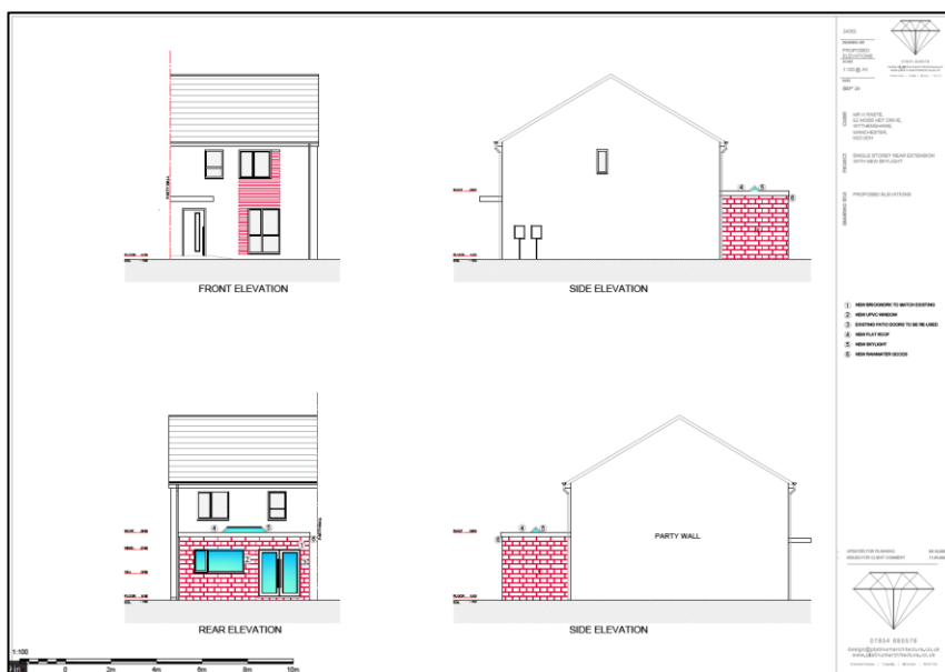
Figure 4. Updated proposed elevations
