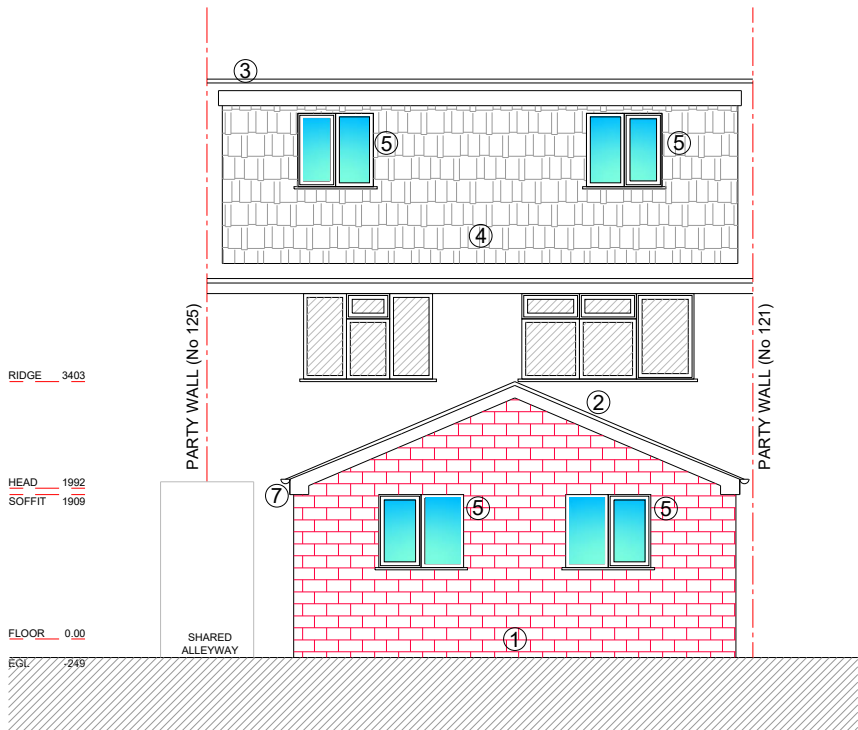
REAR ELEVATION
