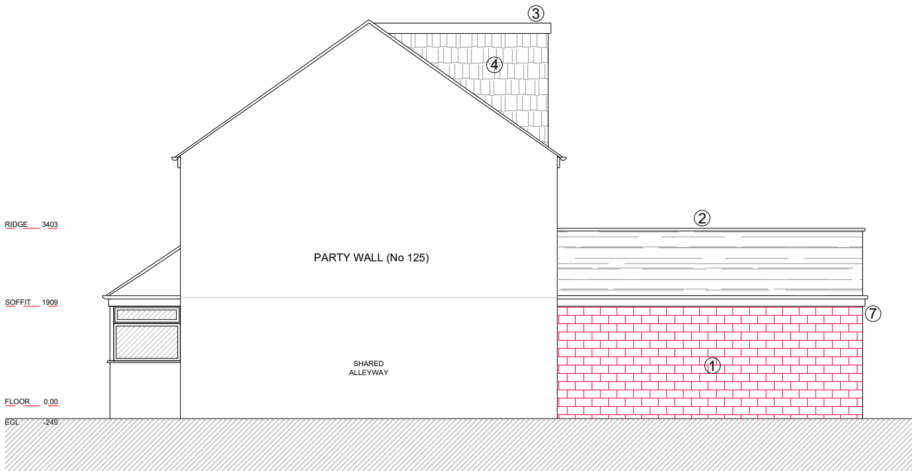
SIDE ELEVATION
