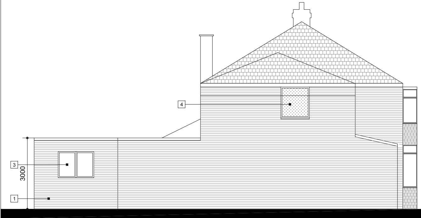
Side Elevation 01
