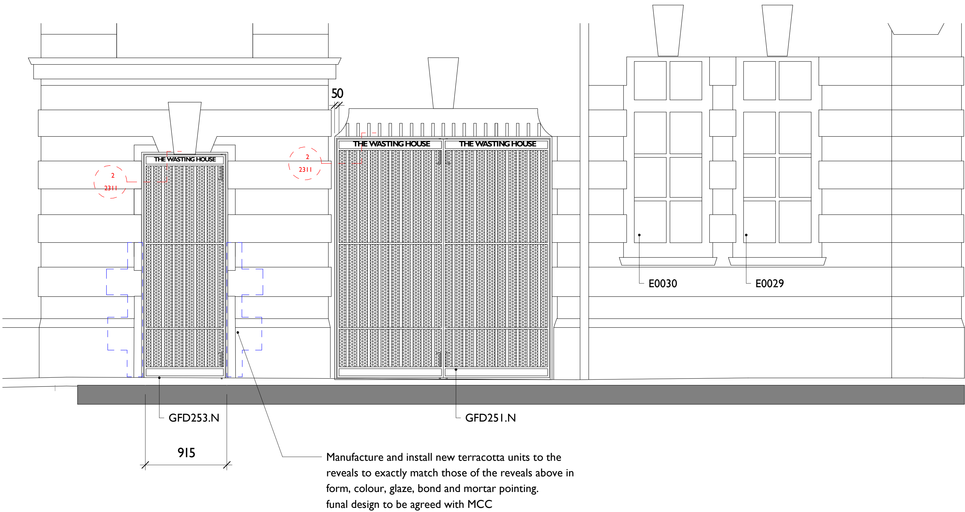
2 2310 Substation Entrance - As Proposed Door Elevation 1 : 25
