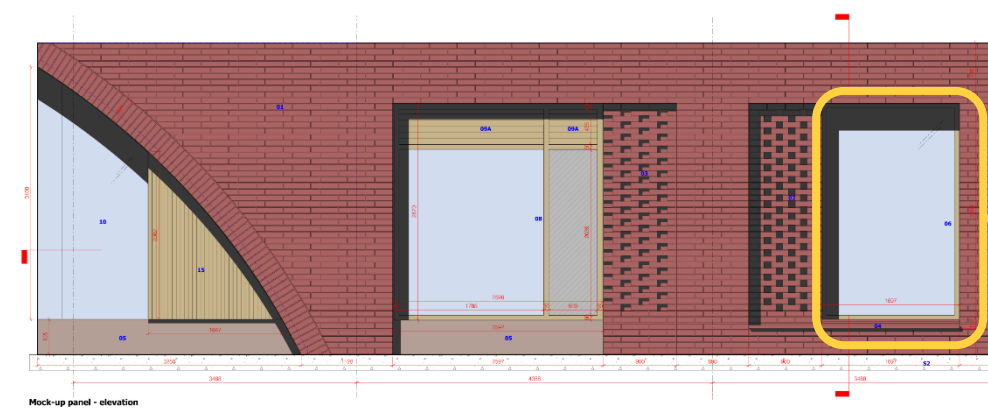
Weep vents to window framing (typical upper floor levels)
