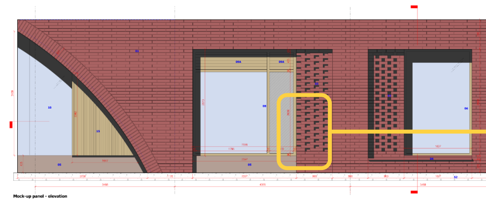
Colour matched mastic between window/ curtain walling framing and brickwork
