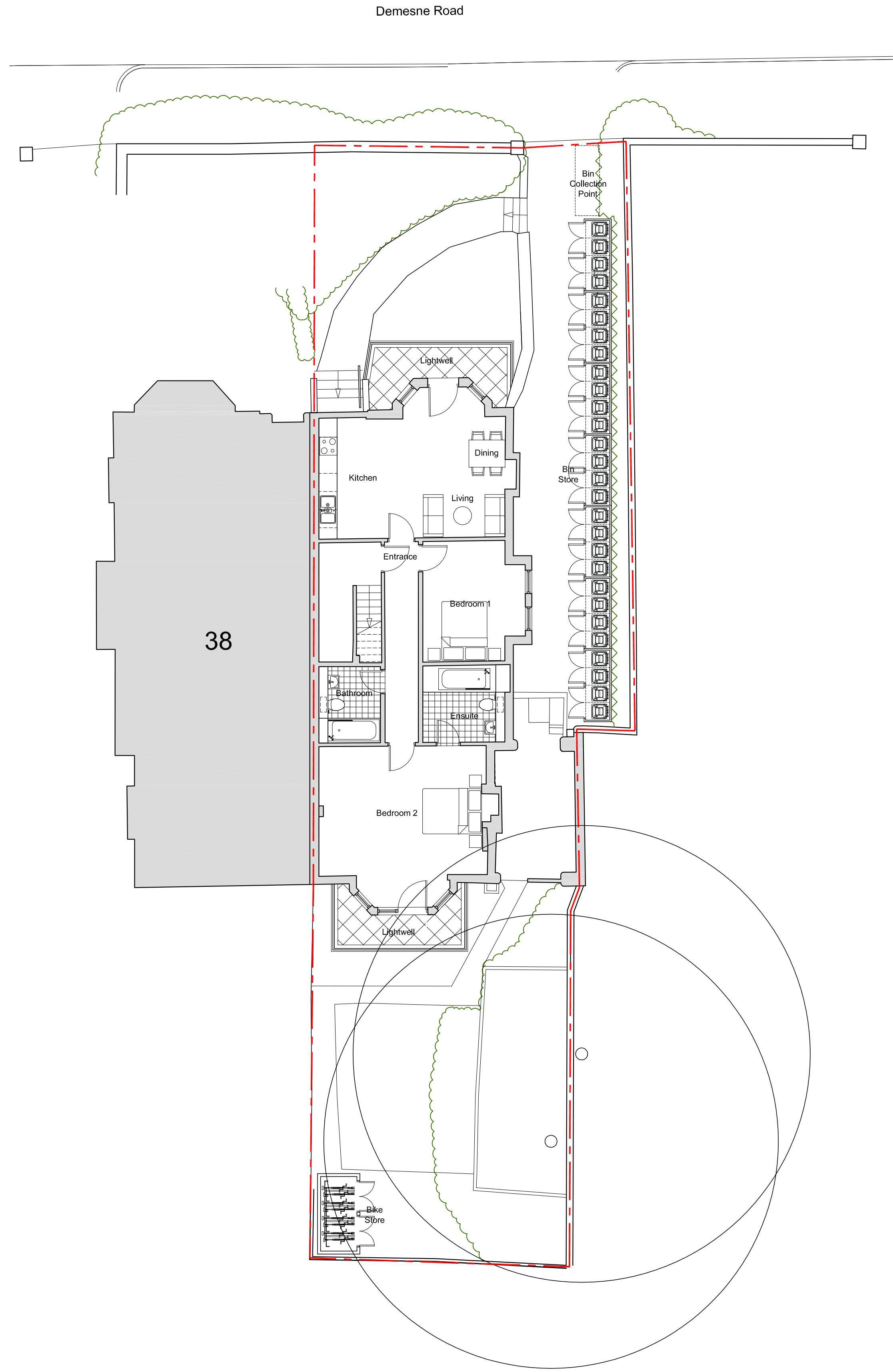
Proposed Lower G/F Plan 1:100
