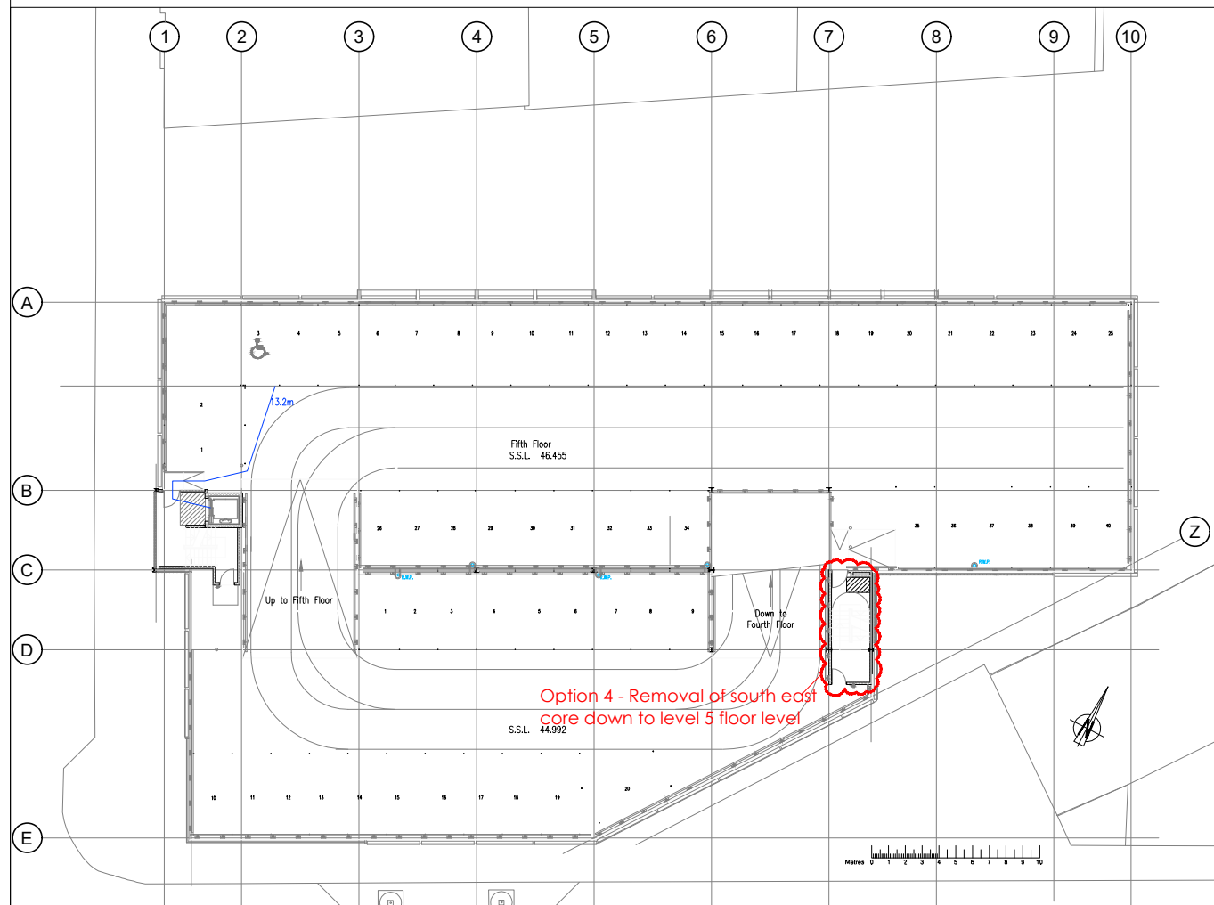
5TH FLOOR PLAN EXISTING
