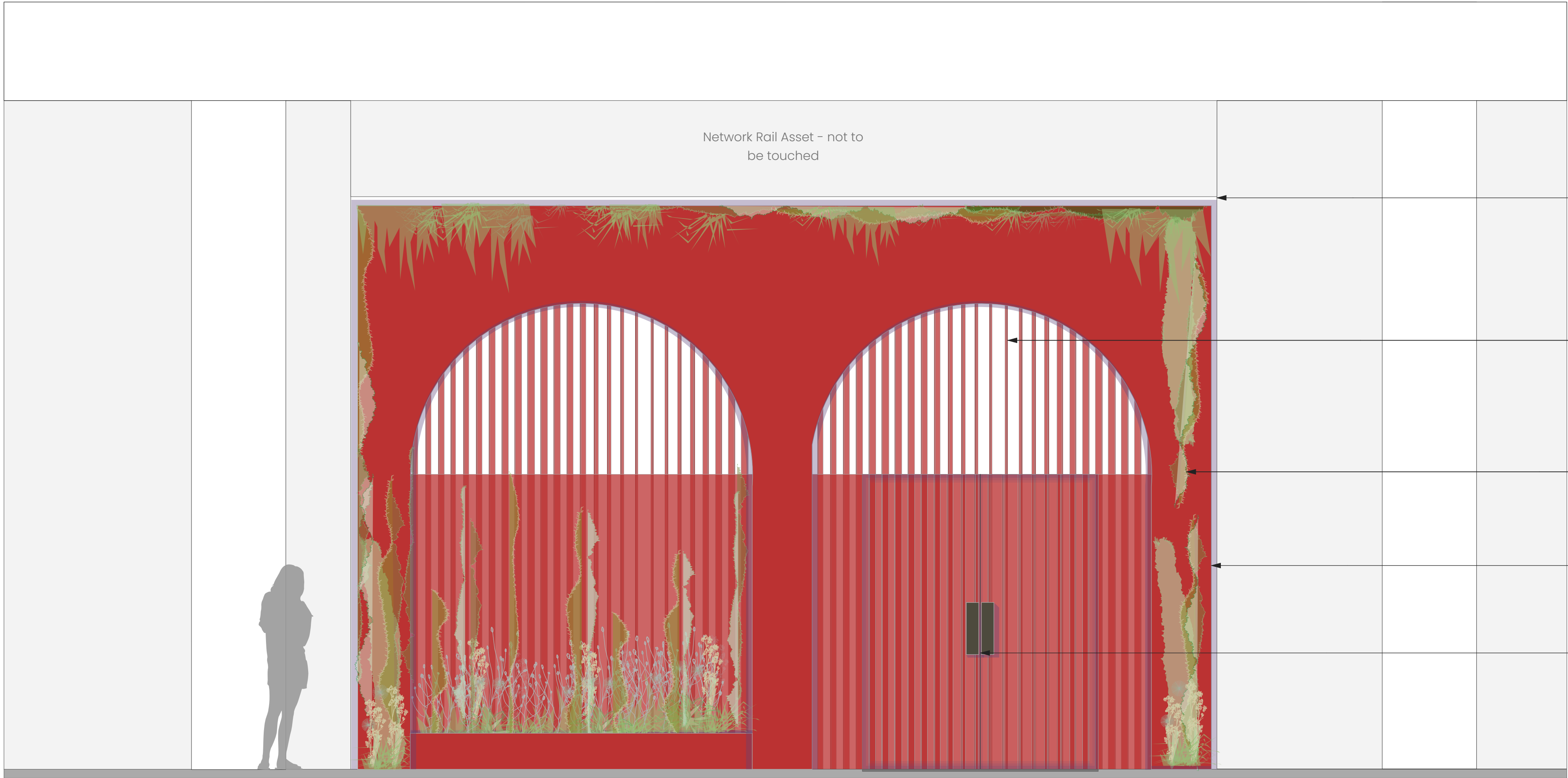
E01 ILLUSTRATIVE ELEVATION Scale: 1:25 @ A1
