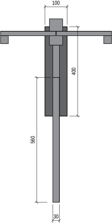
AS PROPOSED - SIDE PROJECTING SIGN
