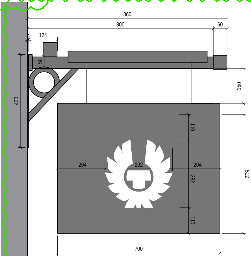
AS PROPOSED - FRONT PROJECTING SIGN
