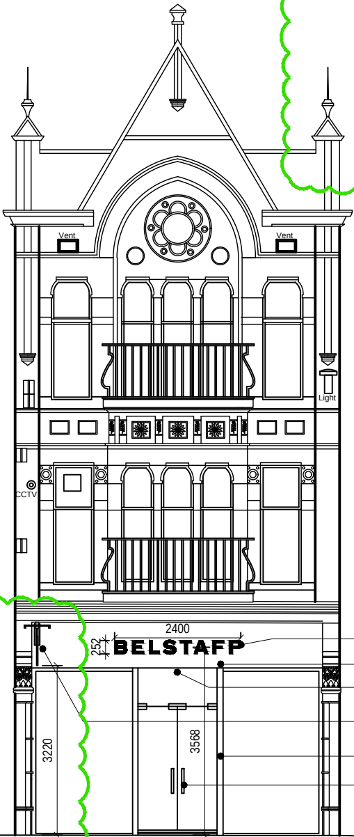
AS PROPOSED - STORE FACADE
