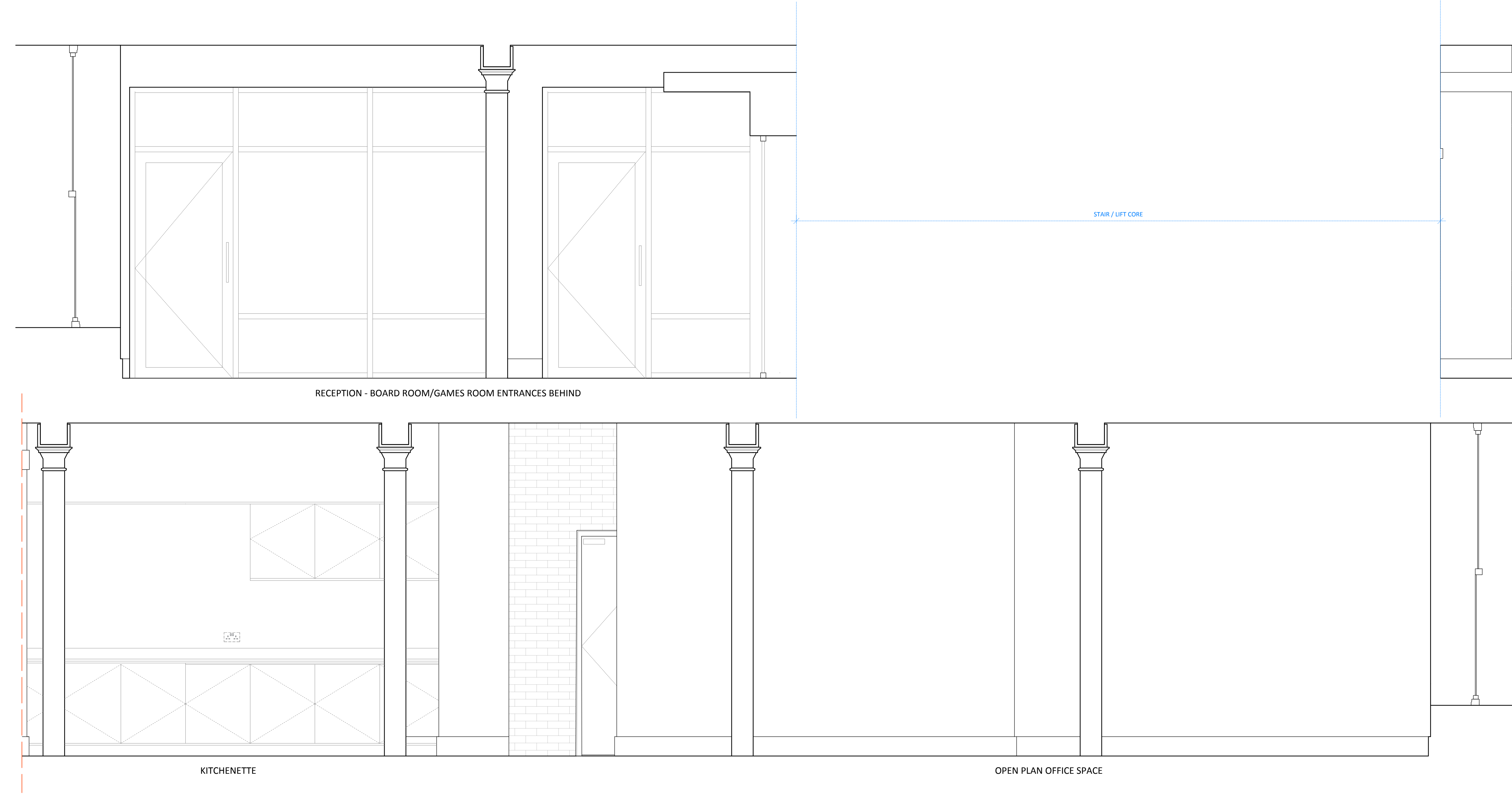
01 Proposed SECTION DD 023 SCALE - 1:20 @ A1 GROUND FLOOR SECTION
