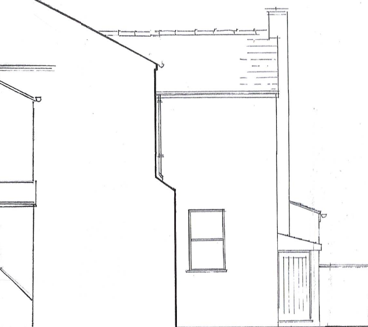
ELEVATION TO N° 8
