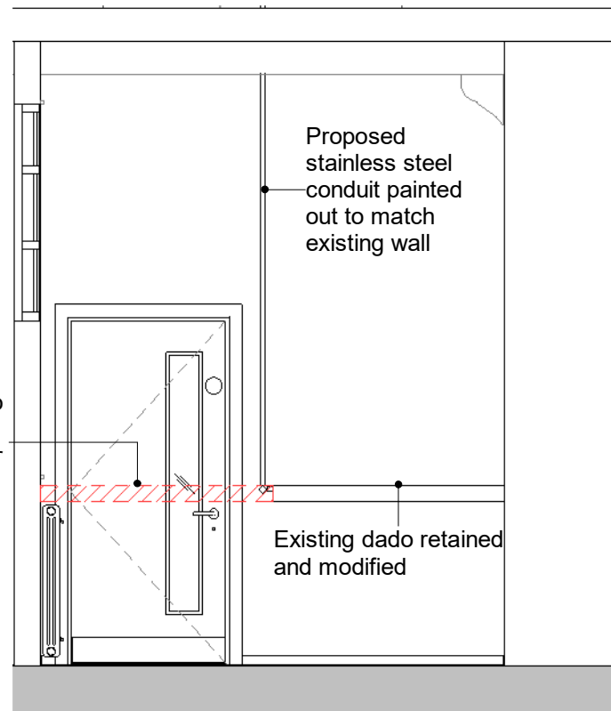
Elevation H
