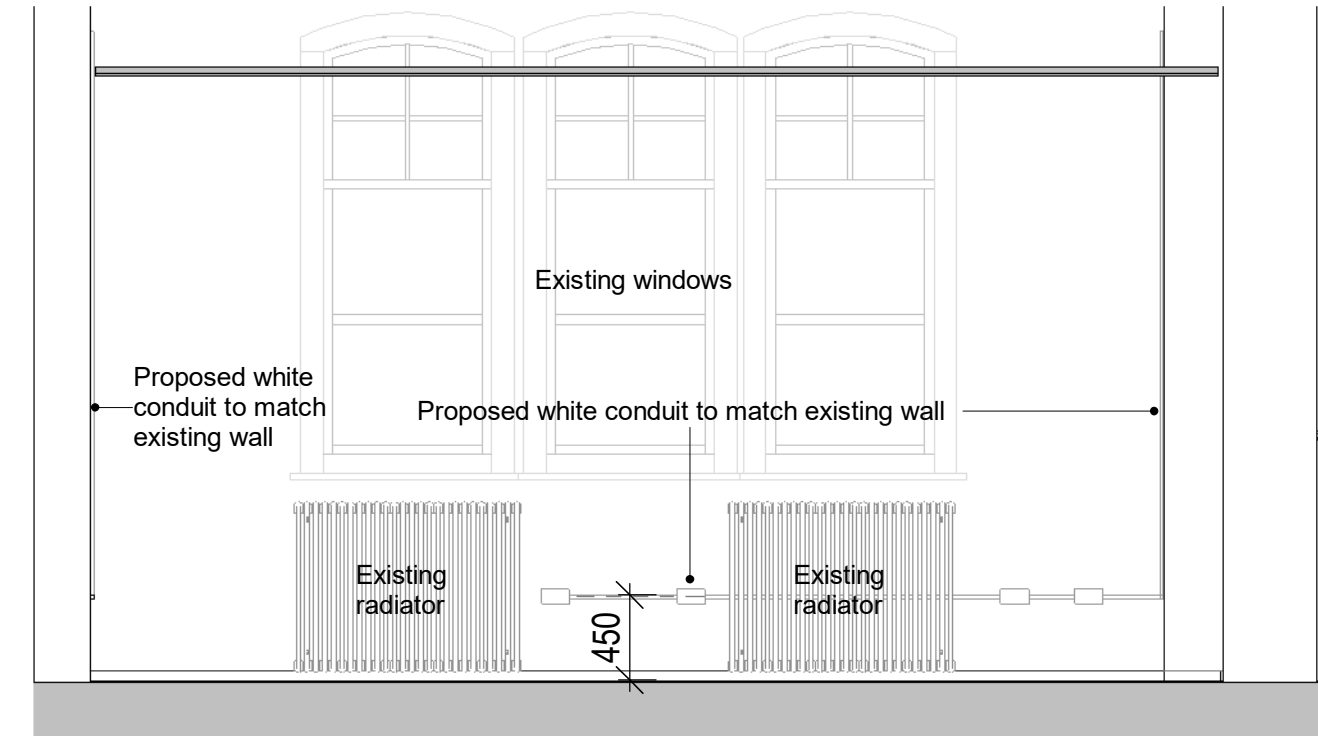
Elevation C
