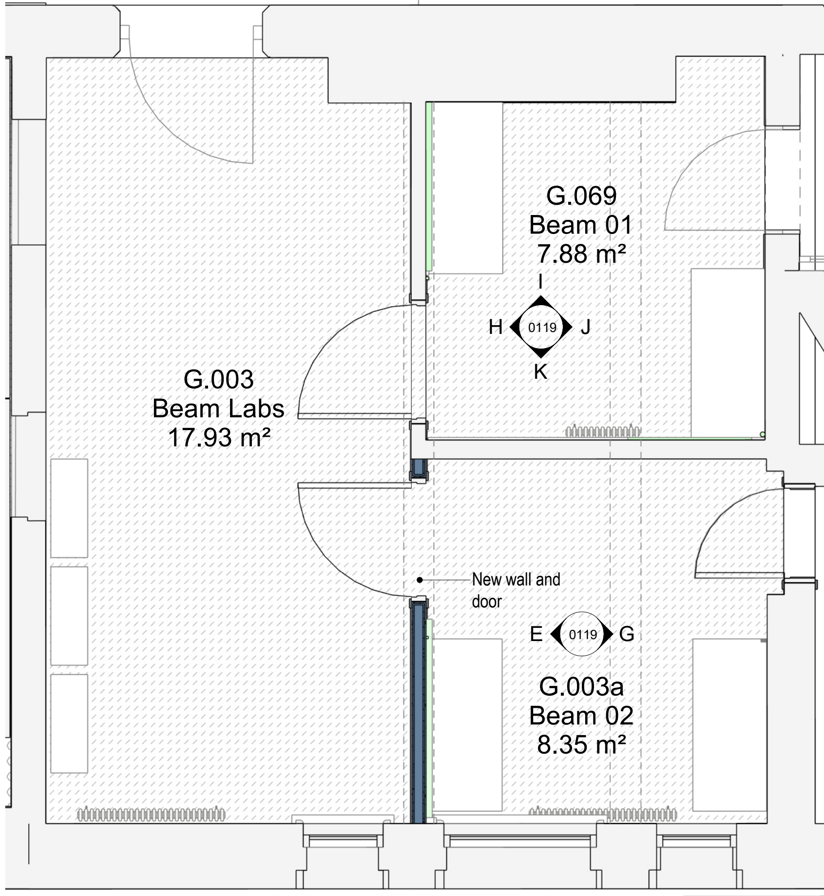
G.003a & G.069 Beam Labs - MEP Location
