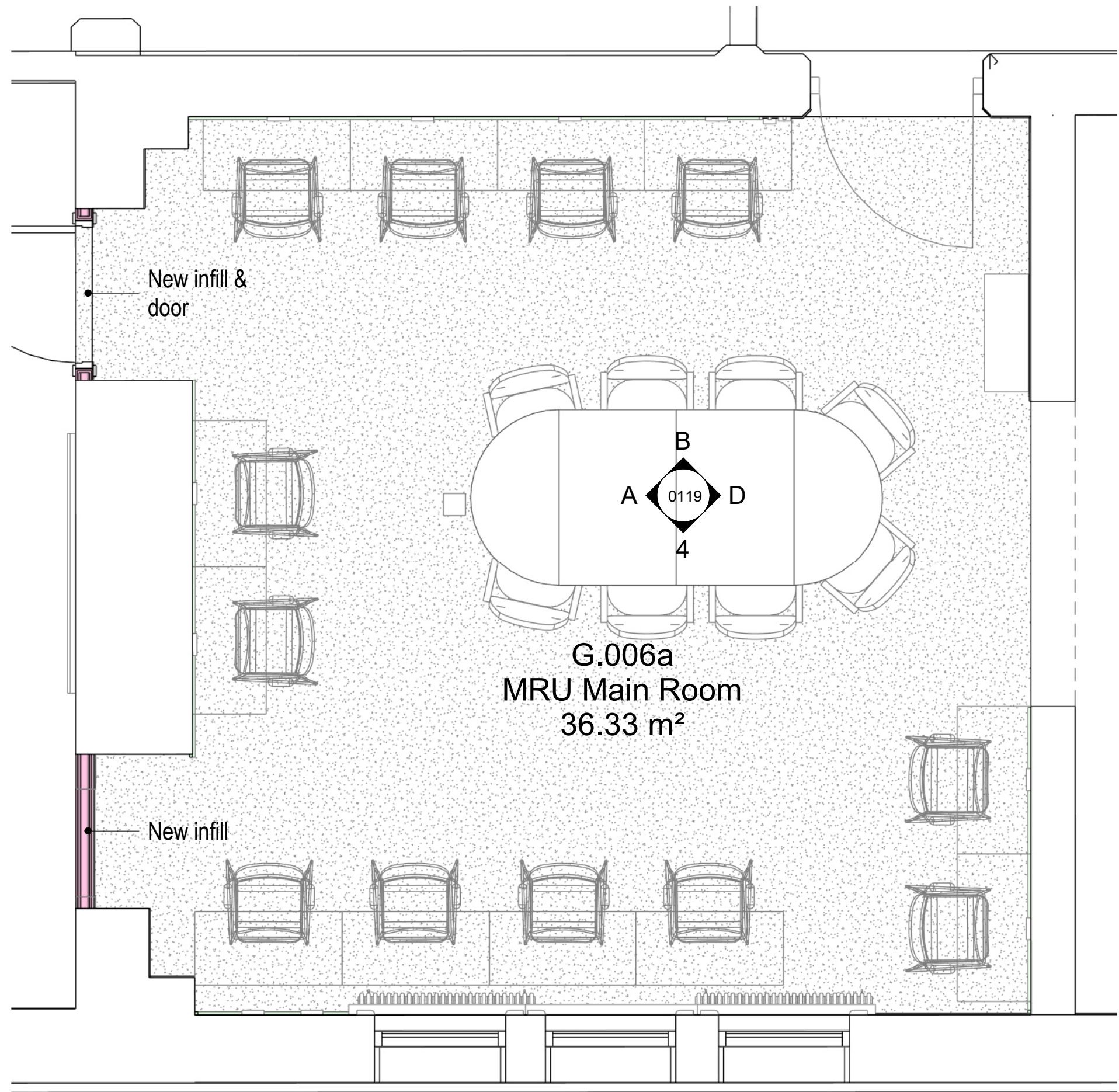
G.006a MRU Main Room - MEP Location
