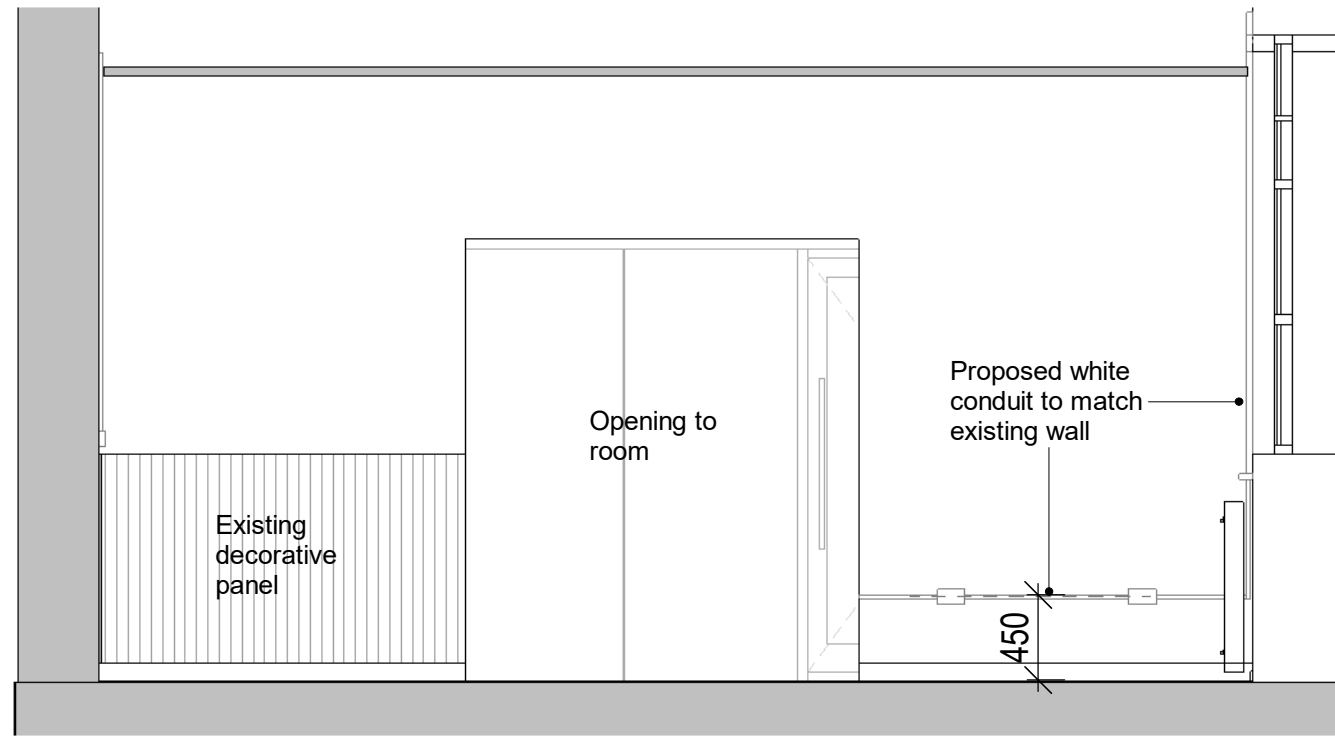
Elevation D
