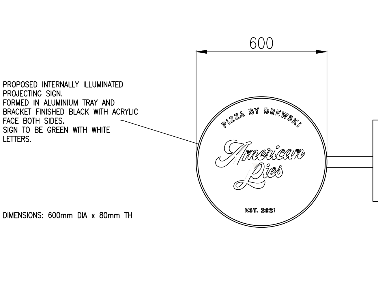
PROPOSED PROJECTING SIGN SCALE 1:10@A1
