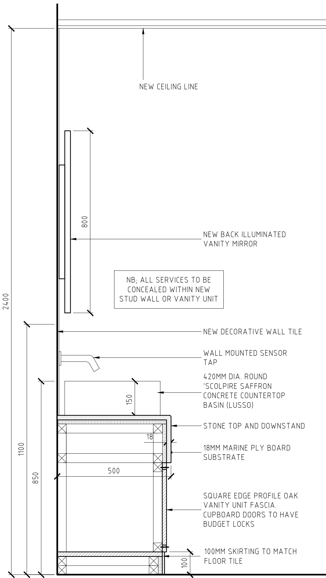
SECTION X-X SCALE 1:10
