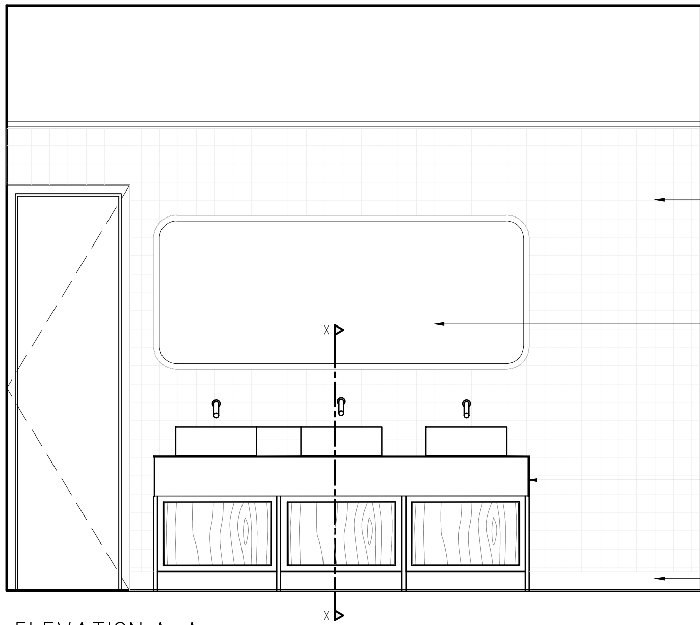
ELEVATION A-A SCALE 1:20
