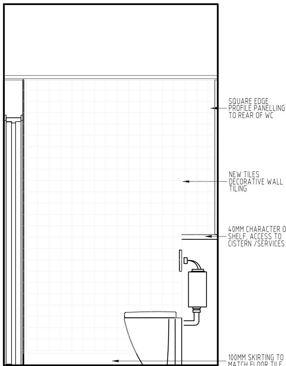
ELEVATION E-E SCALE 1:20
