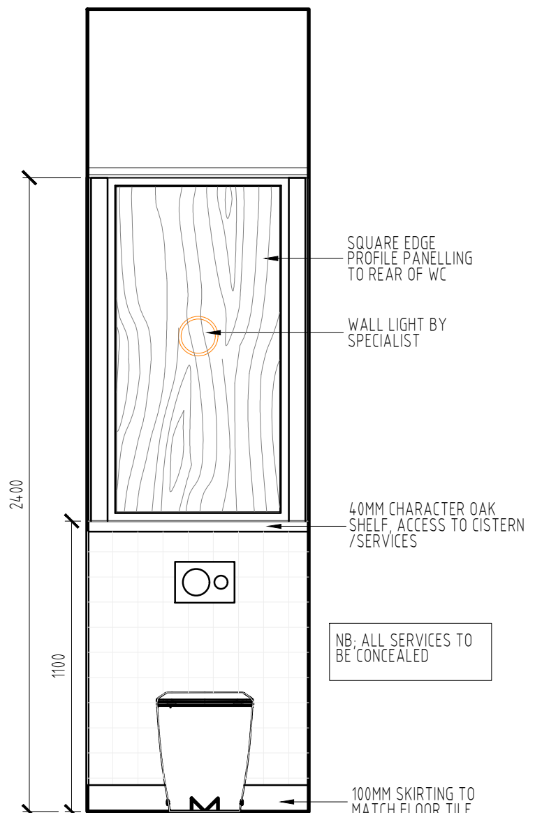
ELEVATION F-F SCALE 1:20
