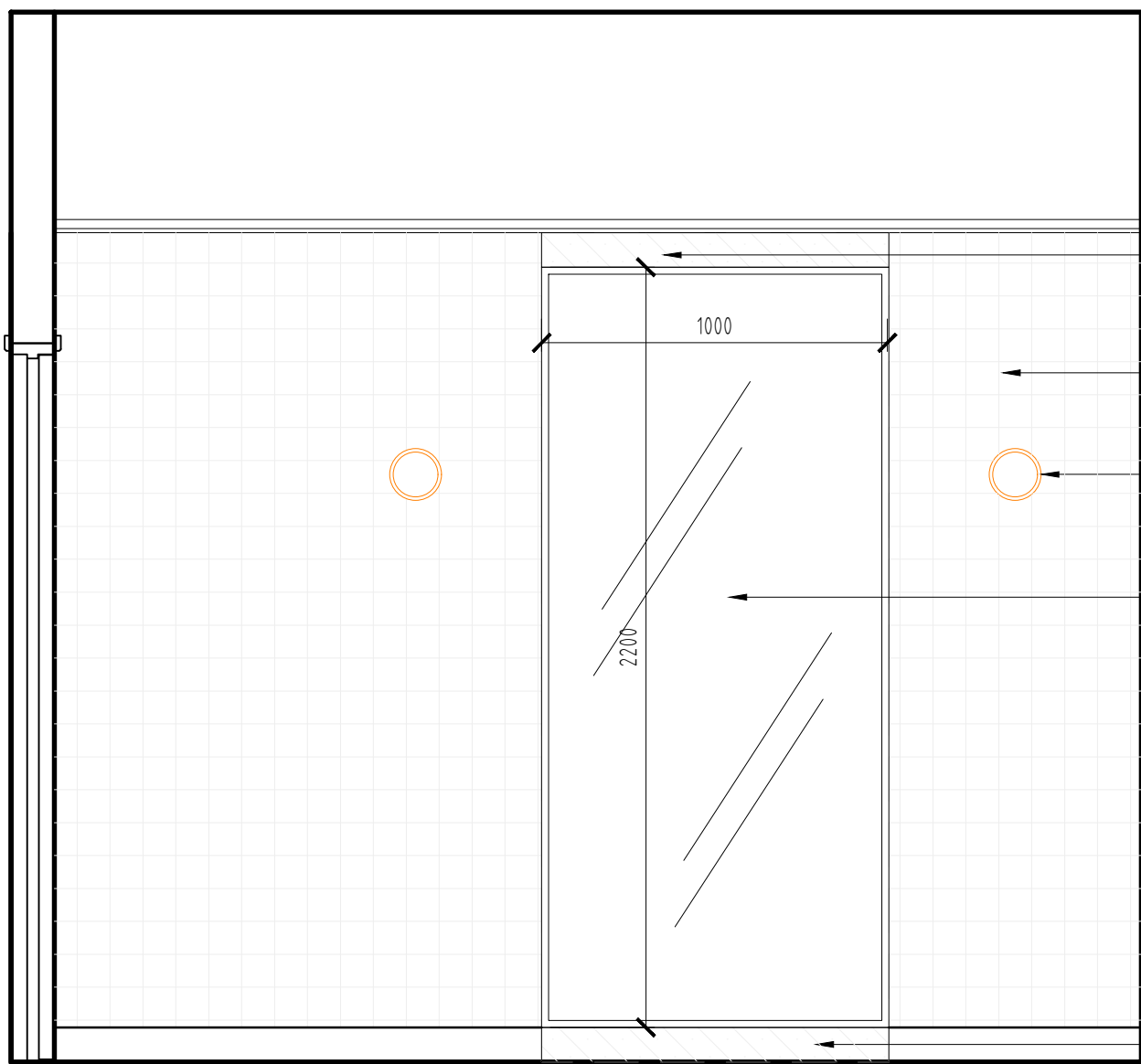
ELEVATION D-D SCALE 1:20
