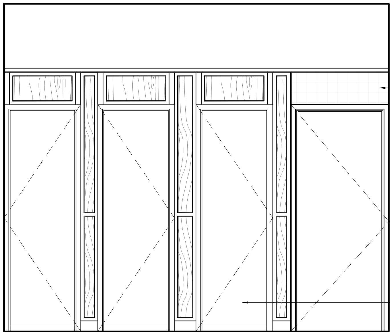
ELEVATION C-C SCALE 1:20
