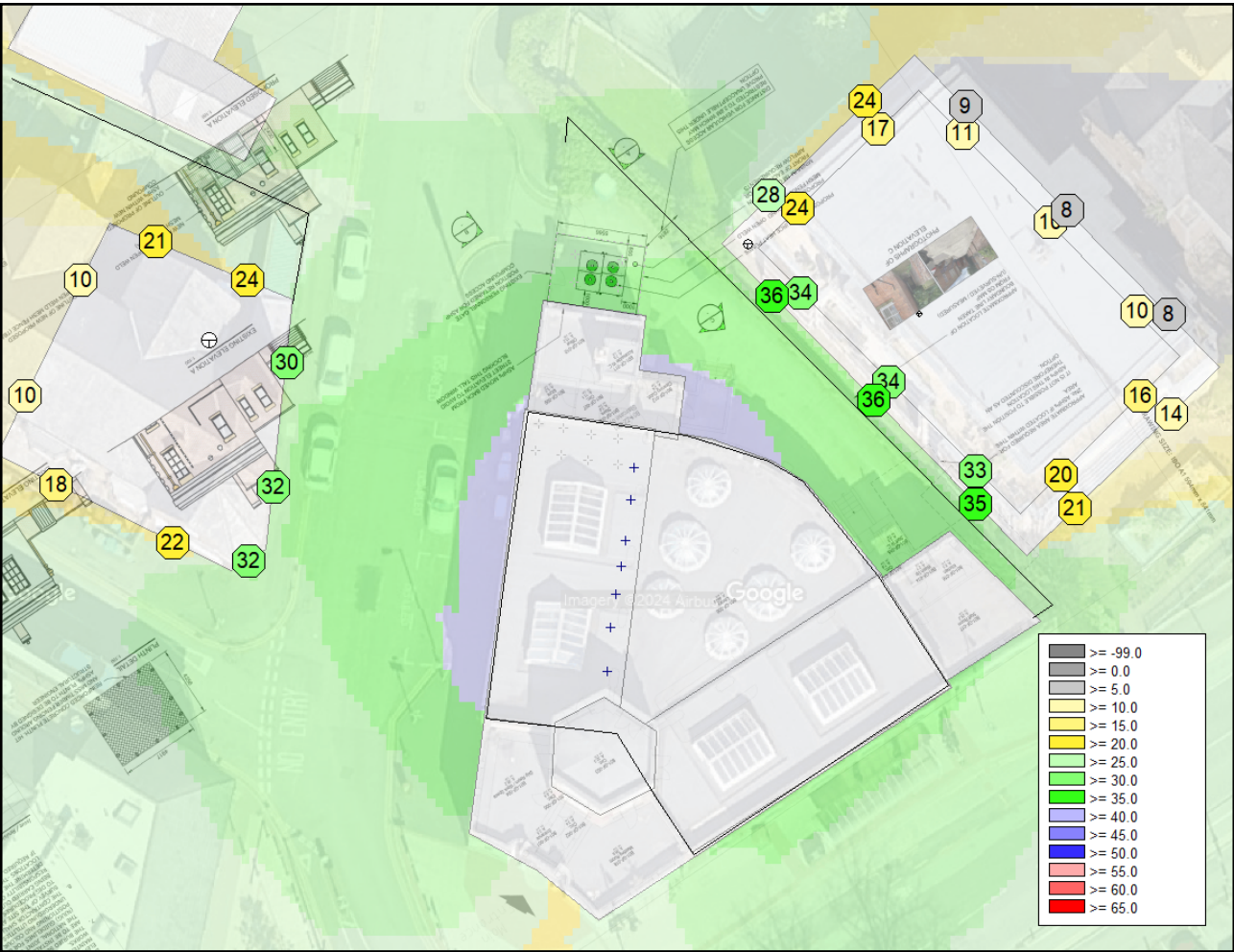
Figure 5.1: Predicted Specific Sound Level (dBA)
