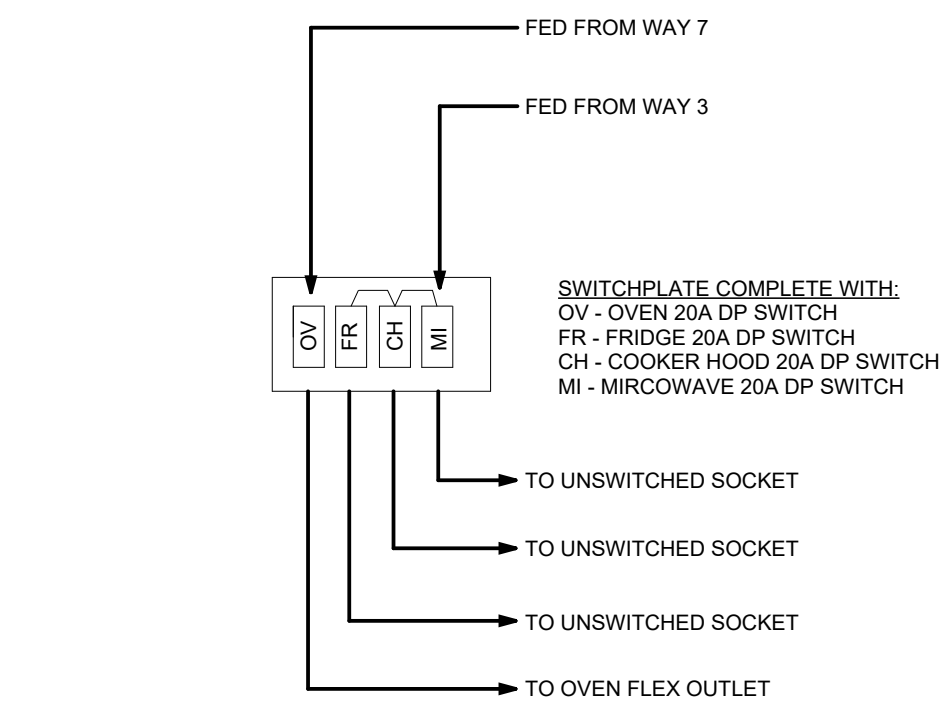
DETAIL A: TYPICAL 4-GANG MULTI-APPLIANCE SWITCHPLATE
