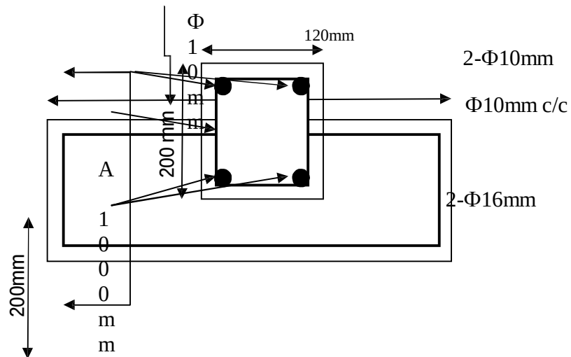
Figure (5) Layout and details of the beam with total length 1000mm
