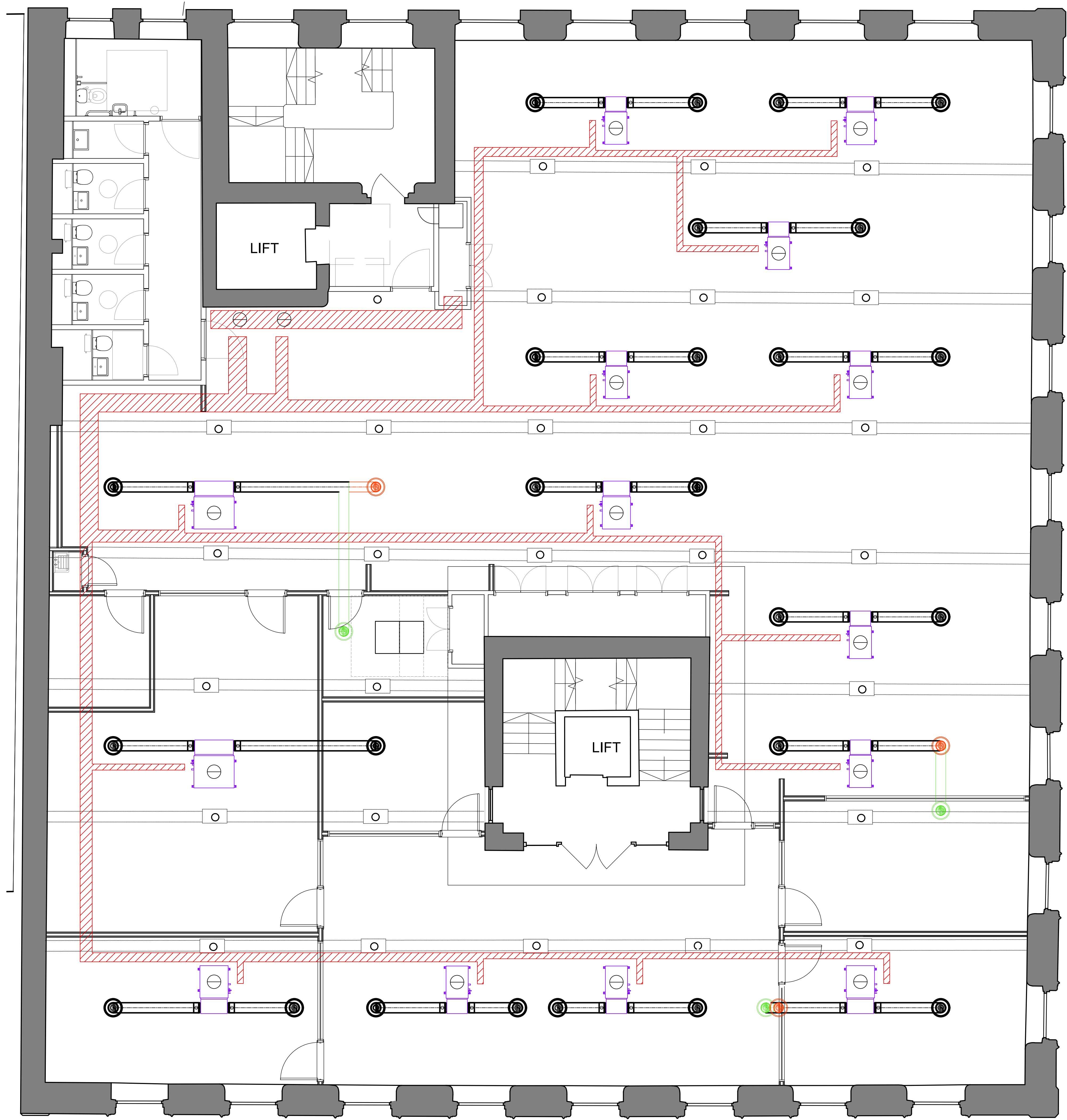
01 FOURTH FLOOR M&E PLAN 305 SCALE - 1:50 @ A1 AS PROPOSED
