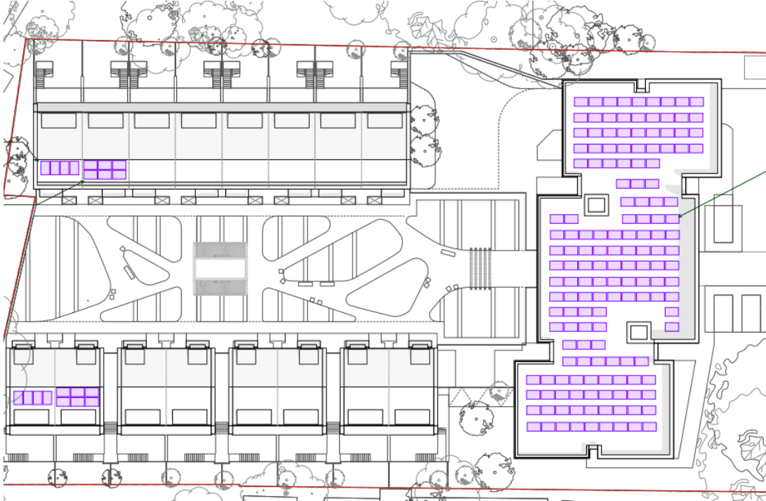
Figure 12 – PV Layout
