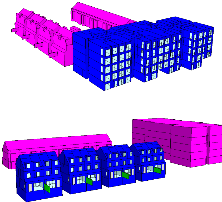
Figure 4 - Views of Dynamic Thermal Model Used to Assess & Mitigate the Risk of Overheating
