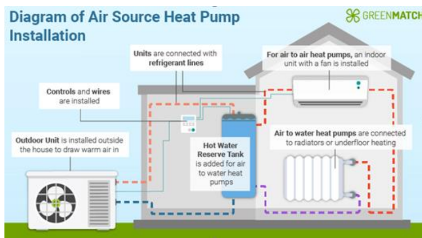
Figure 10 – ASHP Installation
