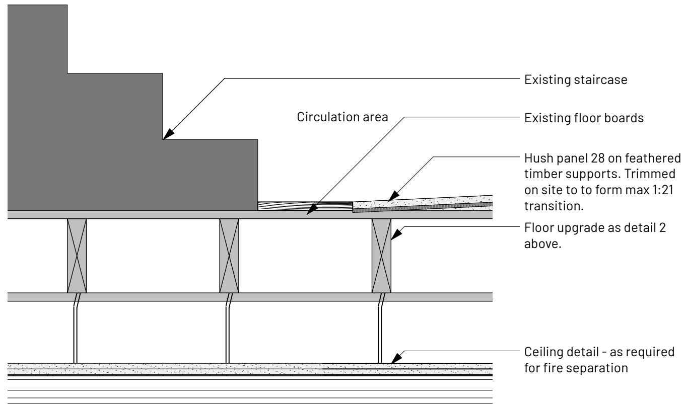
3 Floor transition at existing stair
