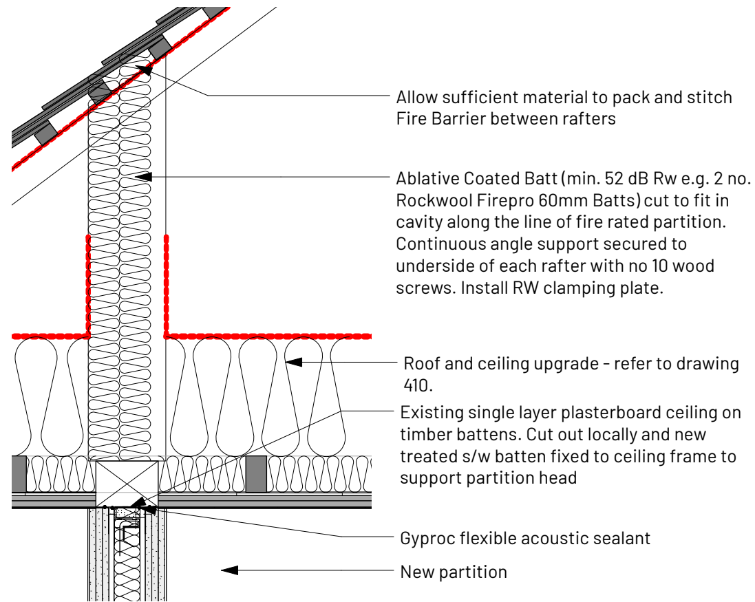
1 Typical Partition - Head/Base
