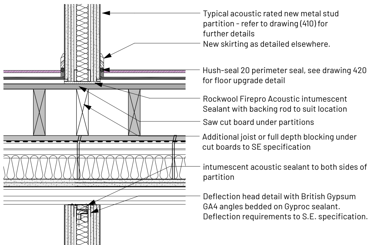
2 Typical Partition - Head/Base
