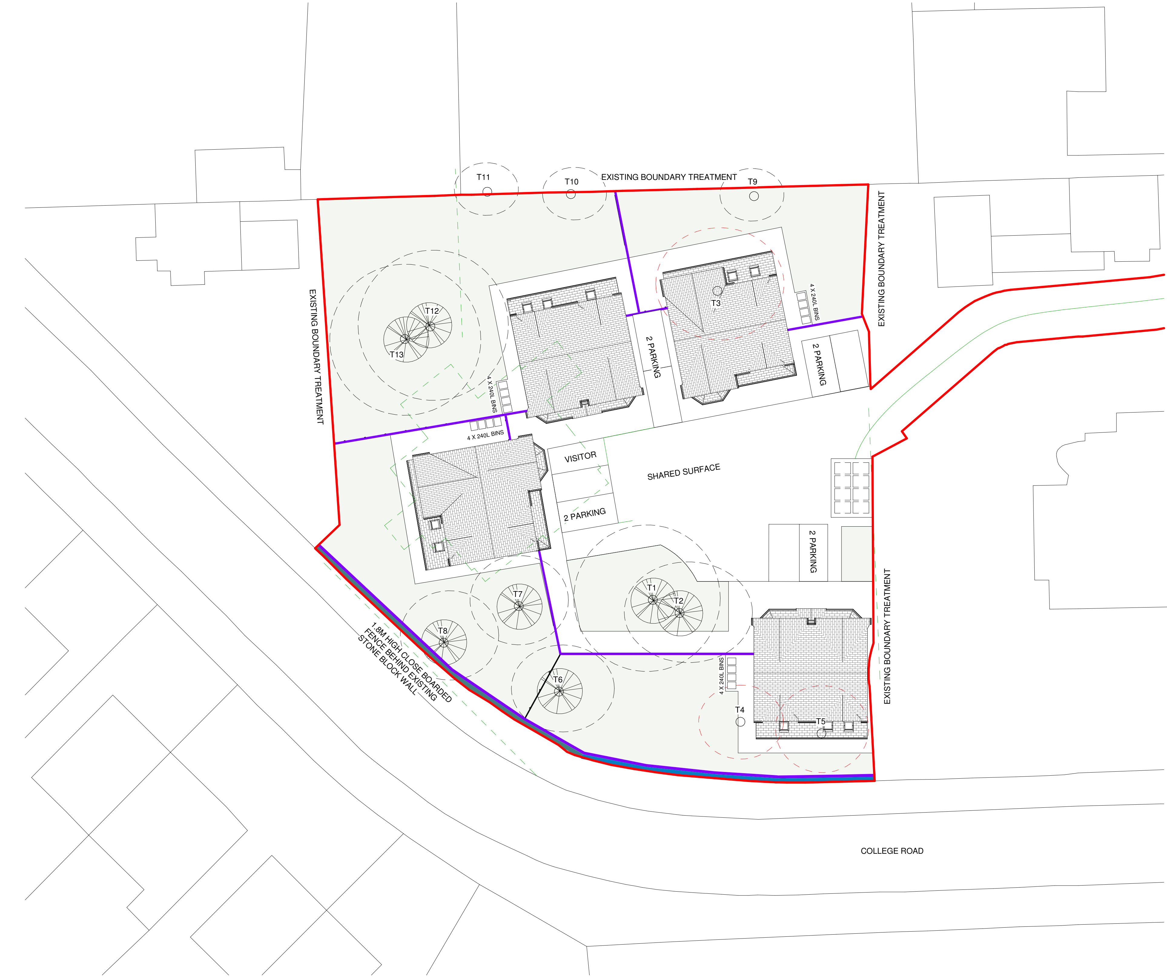
Boundary Plan 1 : 200
