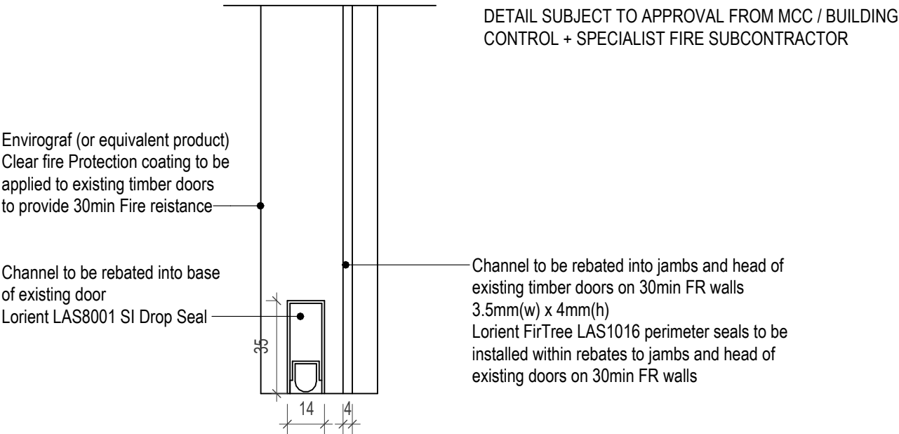
1 Existing Timber door Interventions detail 1 : 2
