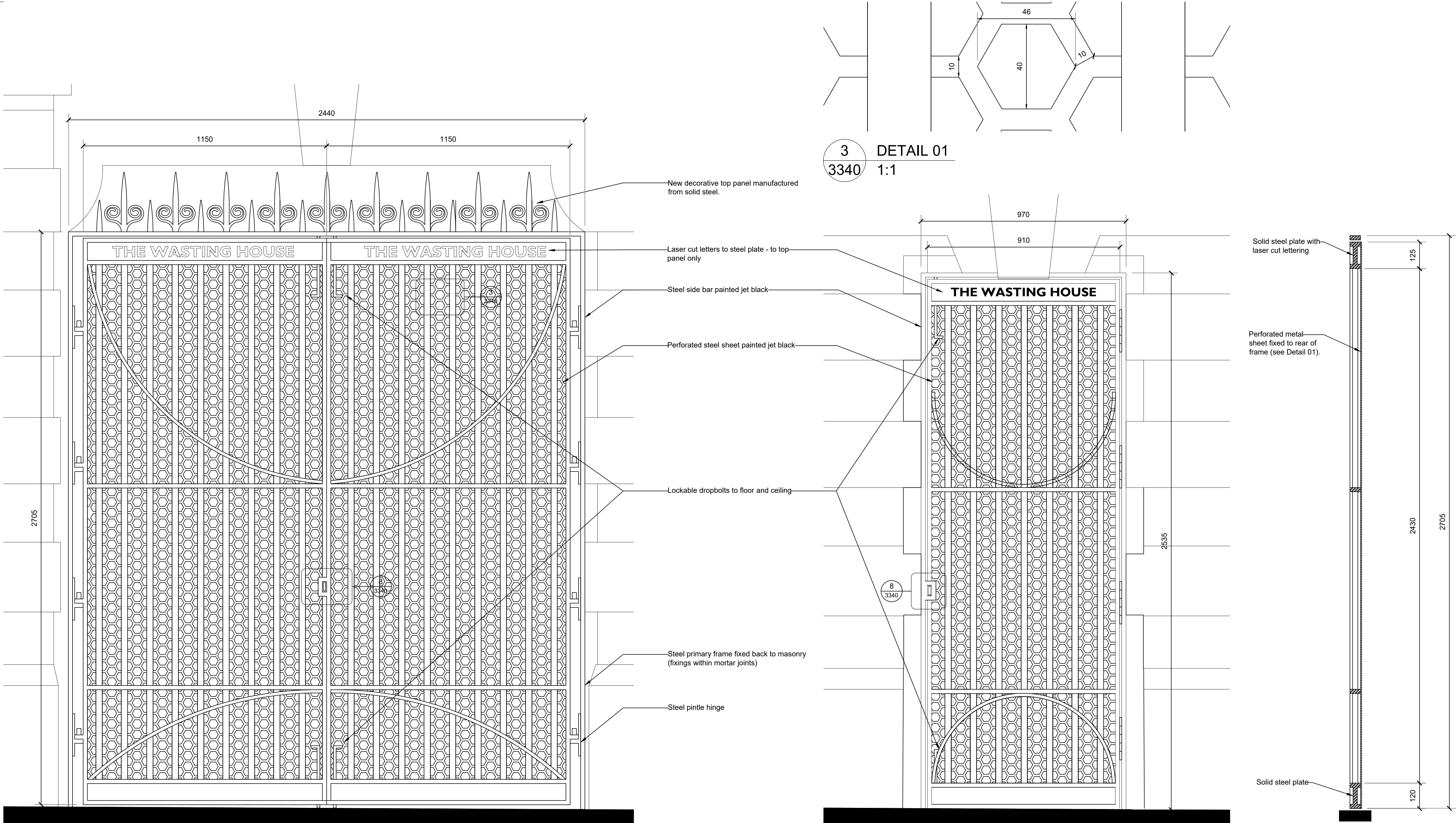
1 GFD293.N(E) - SUBSTATION GATE ELEVATION 01 3340 1:10
