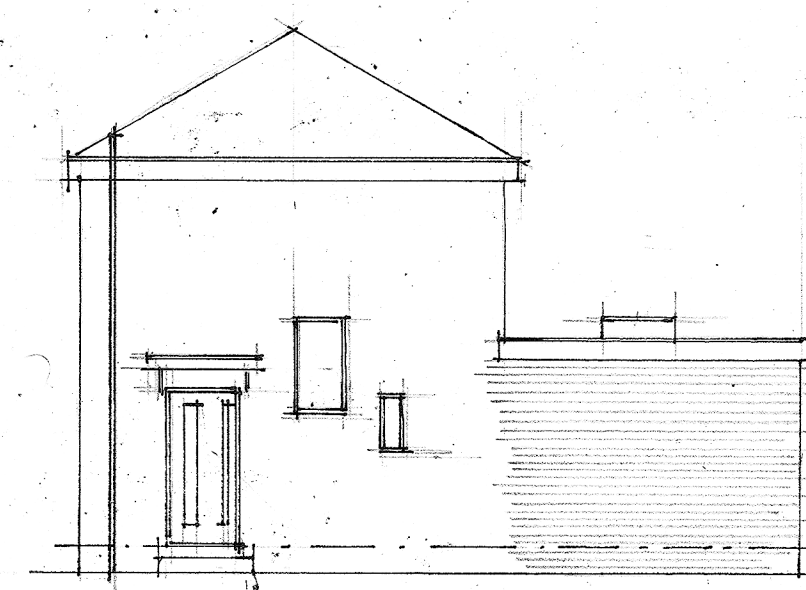
PROPOSED SIDE ELEVATION (to 131)
