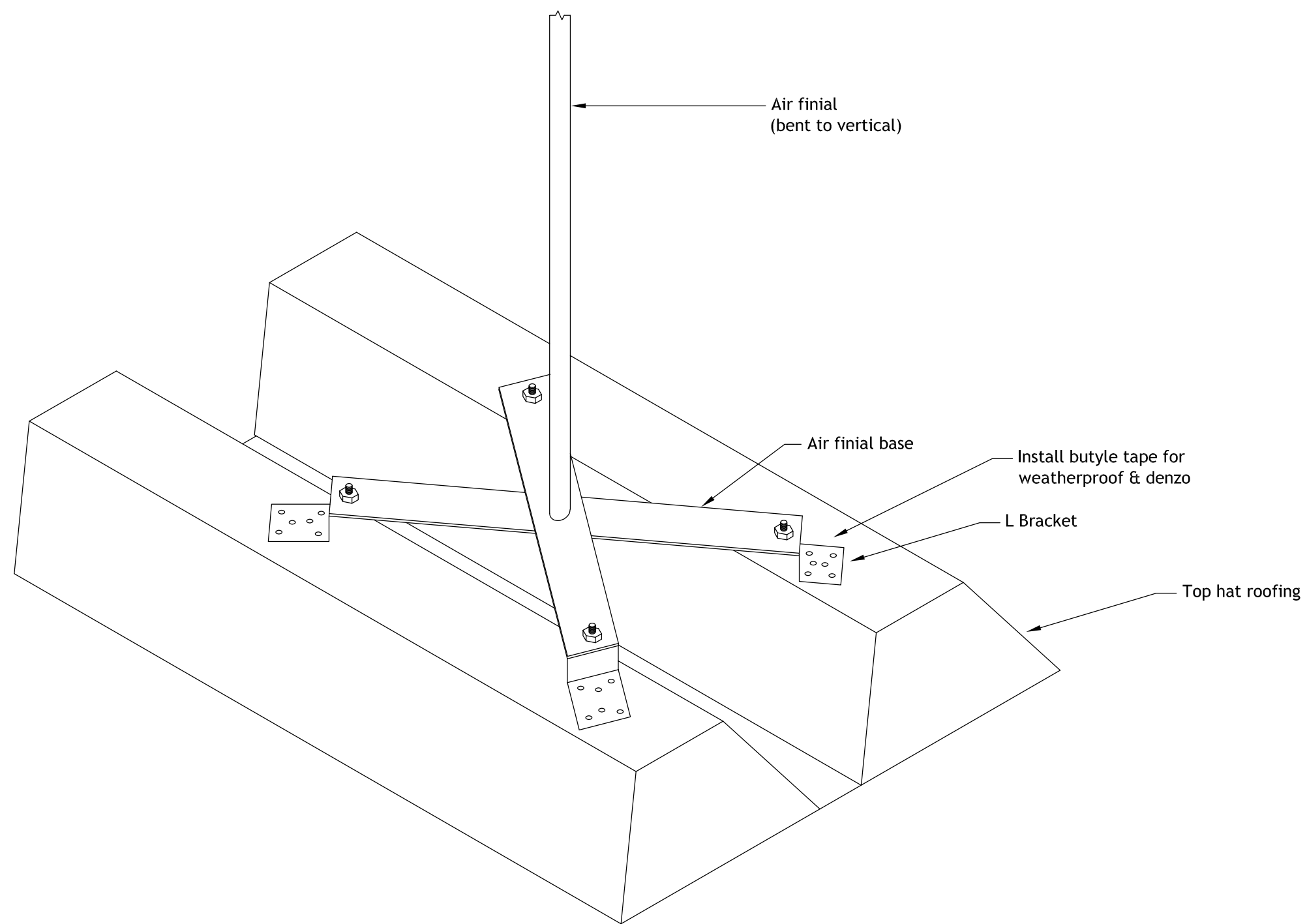
DETAIL 'B' AIR FINIAL MOUNTING
