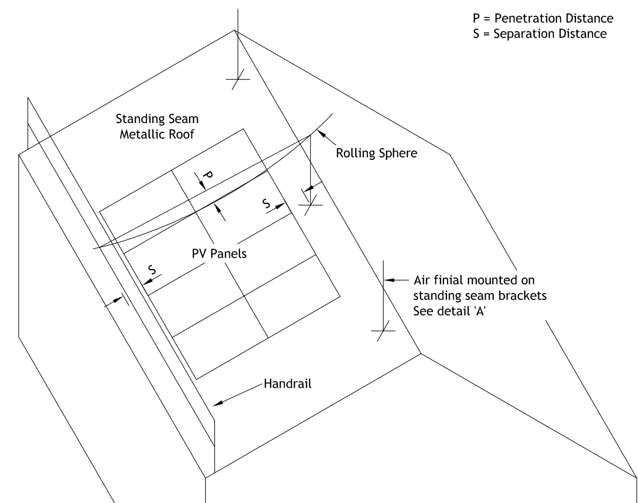
DETAIL 'A' ROLLING SPHERE METHOD OF LIGHTNING PROTECTION
