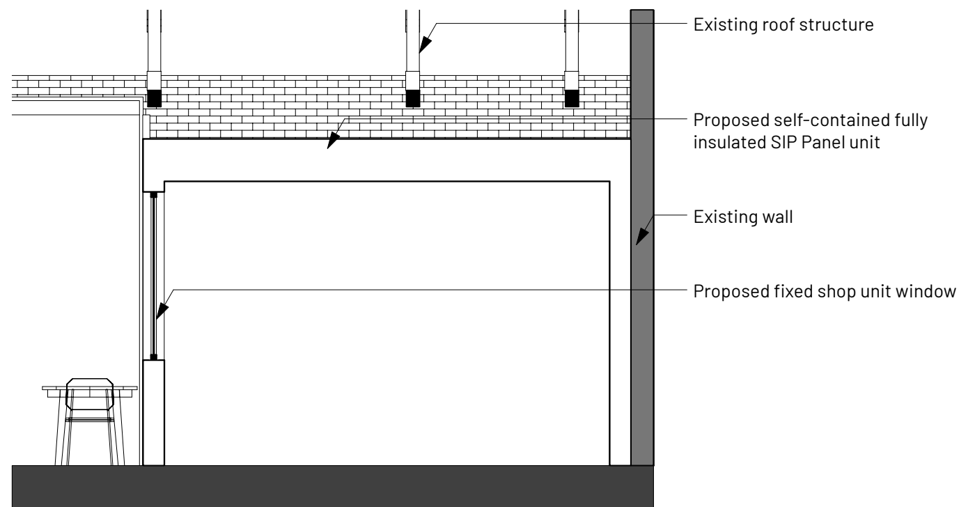
3 Typical Unit/Shop Front Section Scale: 1:50
