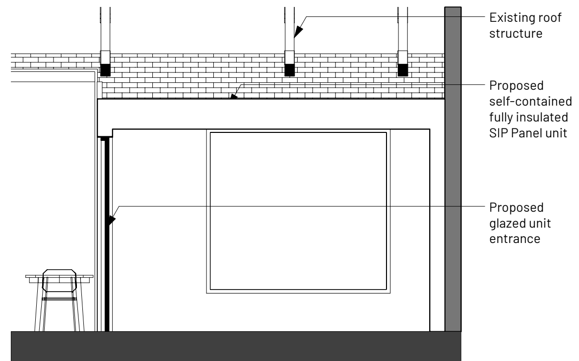
4 Typical Unit Section Scale: 1:50
