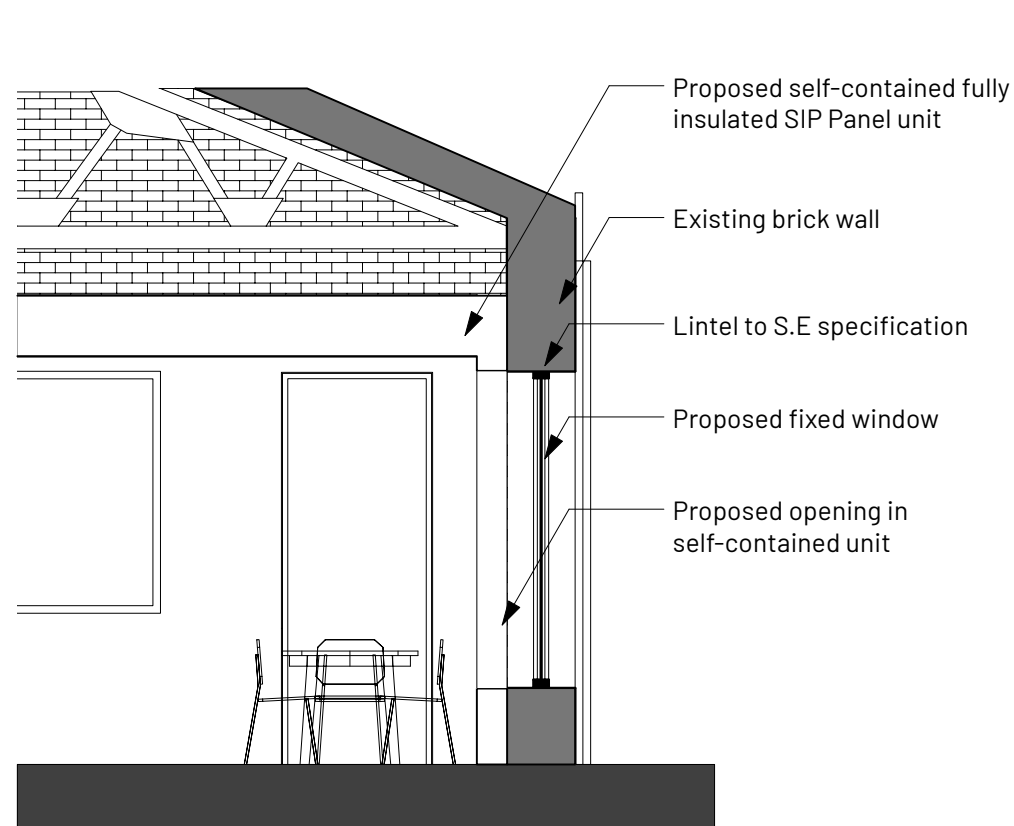
1 Typical Elevation Alteration Section Scale: 1:50
