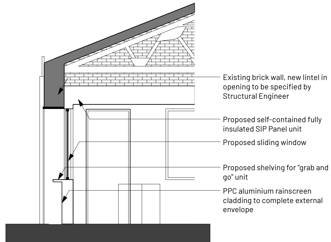
2 Unit 4 - Elevation Alteration Section Scale: 1:50
